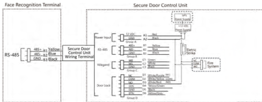
Figure 4-8 Wiring Diagram
