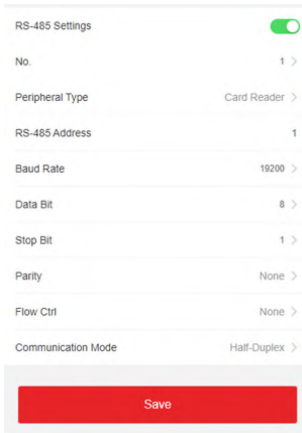
Figure 8-14 RS-485 Page
