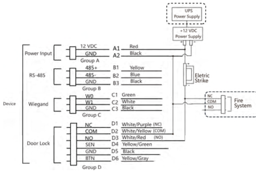
Figure 4-7 Device Wiring
