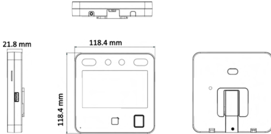
Figure D-1 Dimension (With Fingerprint)
