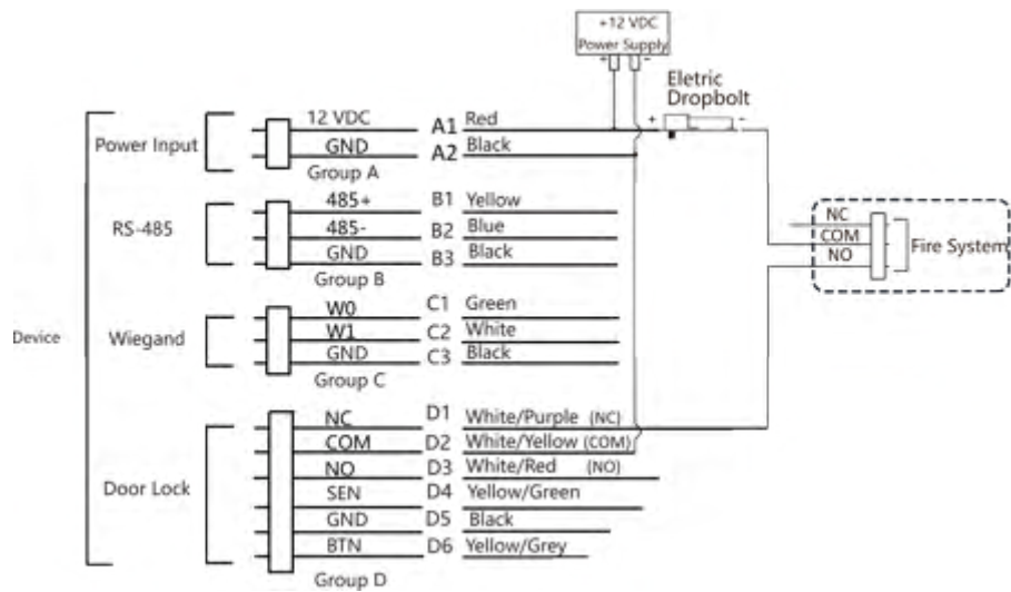
Figure 4-5 Wiring Device
