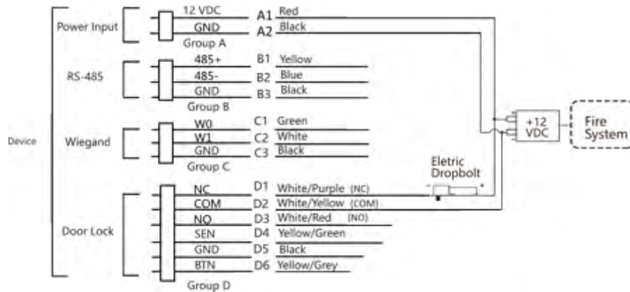
Figure 4-3 Wire Device
