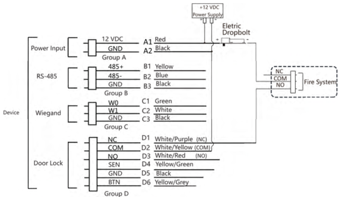
Figure 4-5 Wiring Device
