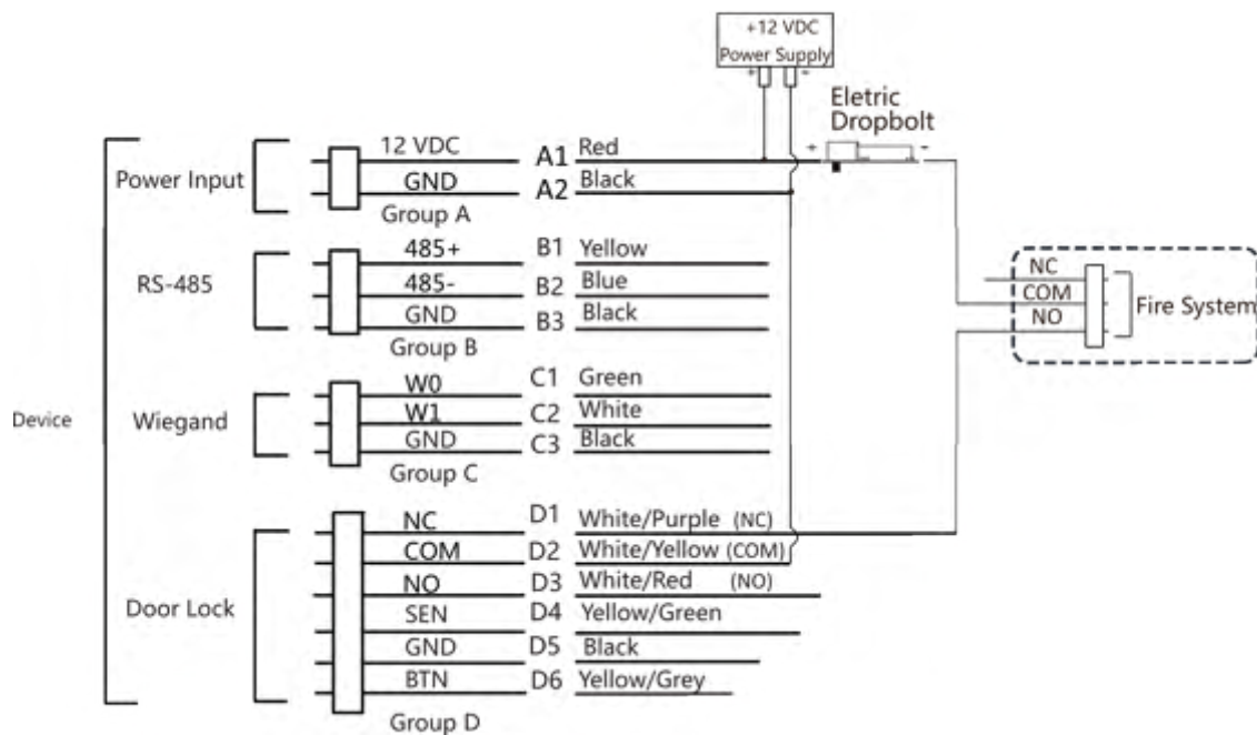
Figure 4-5 Wiring Device
