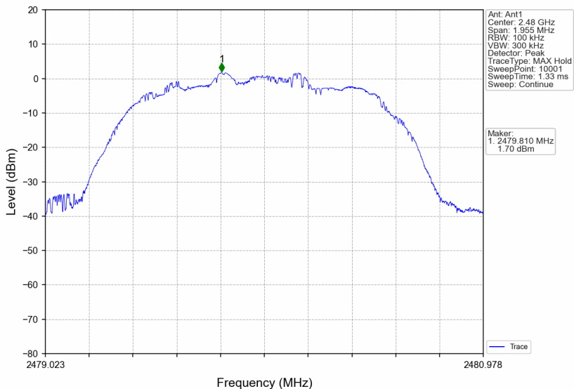
8DPSK_3DH5_HCH_2480MHz_Ant1_NTNV
