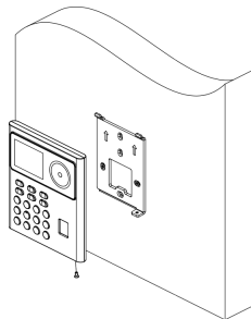
Figure 3-8 Hang Device
