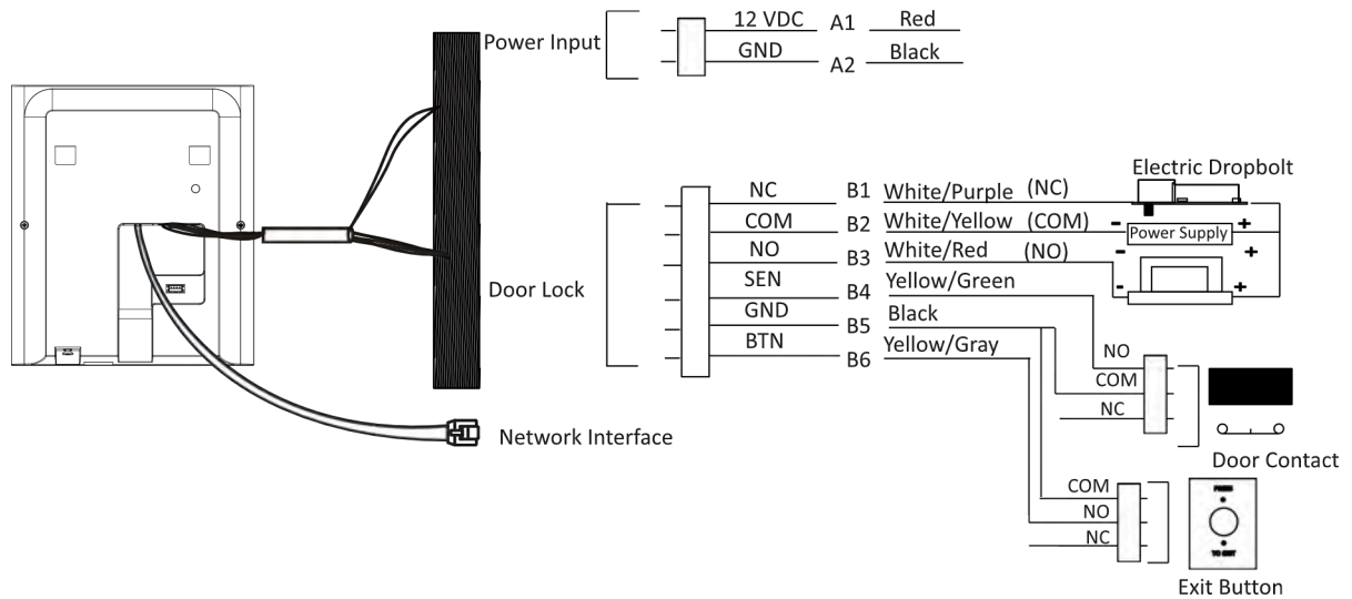
Figure 4-1 Device Wiring
