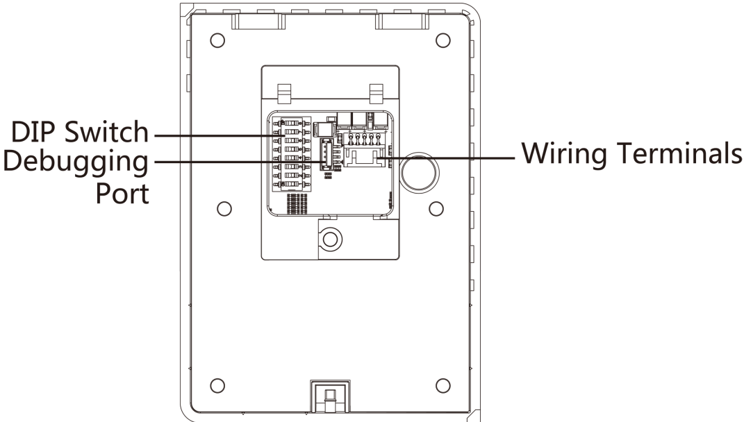
Figure 2-2 Rear View
