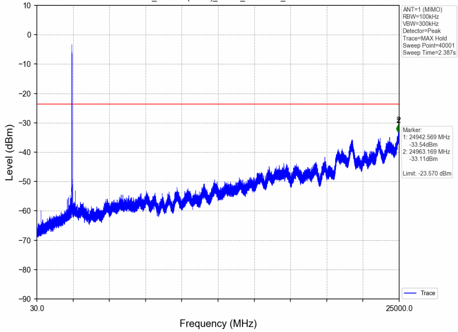
Unwanted Emissions in Non-restricted Frequency Bands NTNV_802.11n(HT40)_MIMO_2452MHz_ANT1
