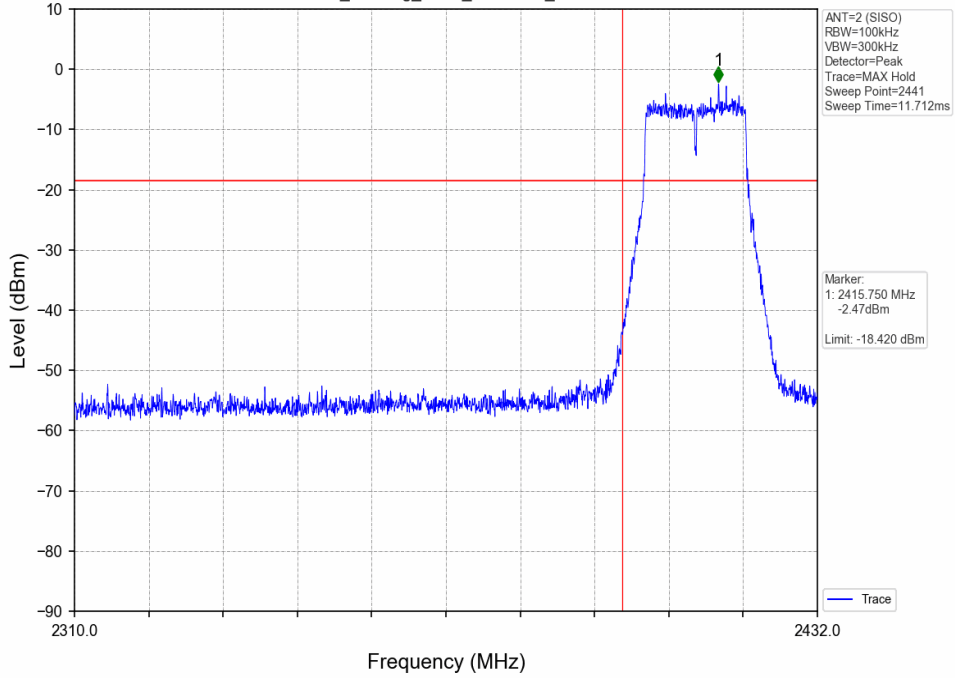
Unwanted Emissions in Non-restricted Frequency Bands NTNV_802.11g_SISO_2412MHz_ANT2
