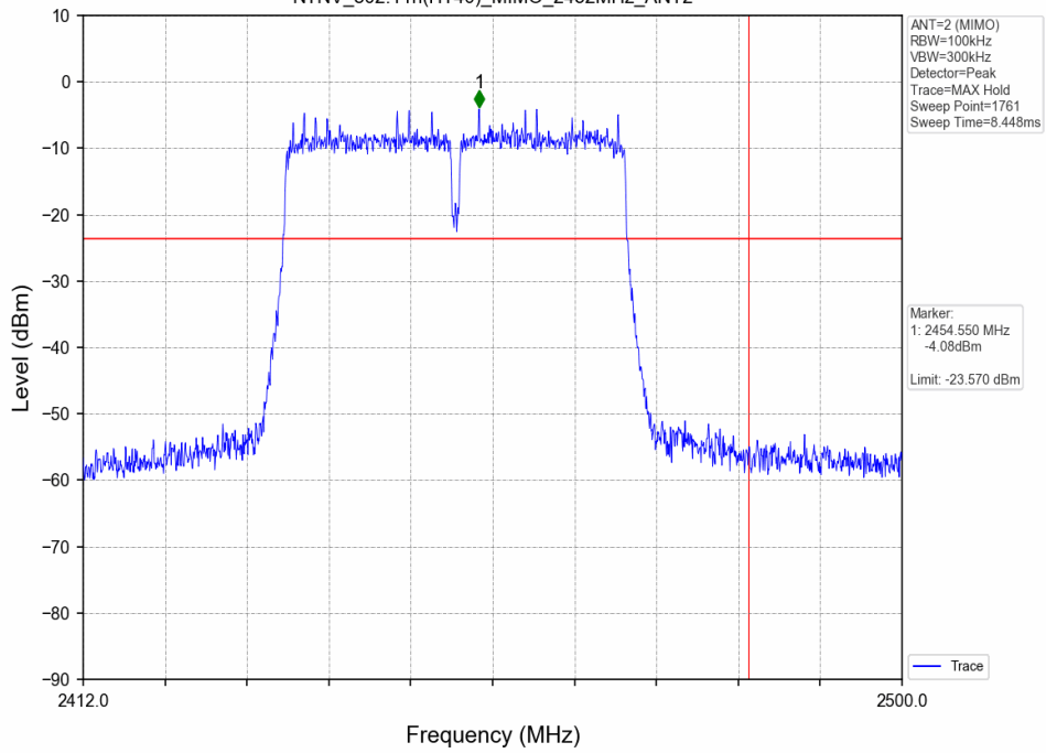
Unwanted Emissions in Non-restricted Frequency Bands NTNV_802.11n(HT40)_MIMO_2452MHz_ANT2
