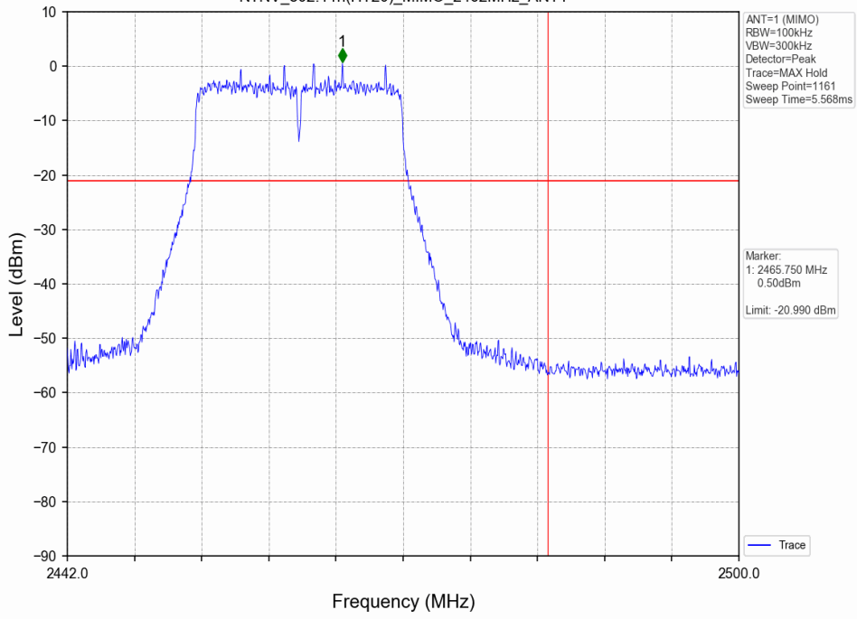
Unwanted Emissions in Non-restricted Frequency Bands NTNV_802.11n(HT20)_MIMO_2462MHz_ANT1
