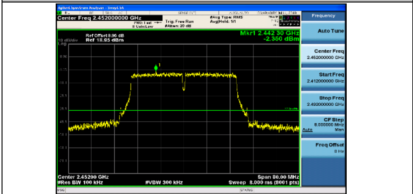
RF Conducted Spurious Emissions_11N40ISO_2452_Ant2
