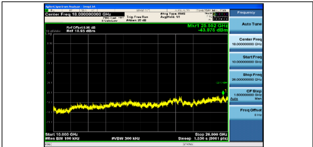
RF Conducted Spurious Emissions_11N40ISO_2437_Ant2
