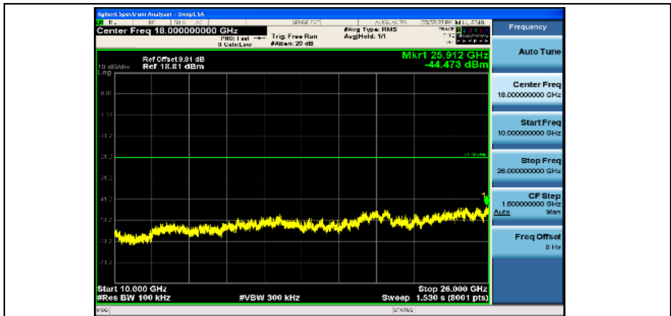
RF Conducted Spurious Emissions_11B_2437_Ant2
