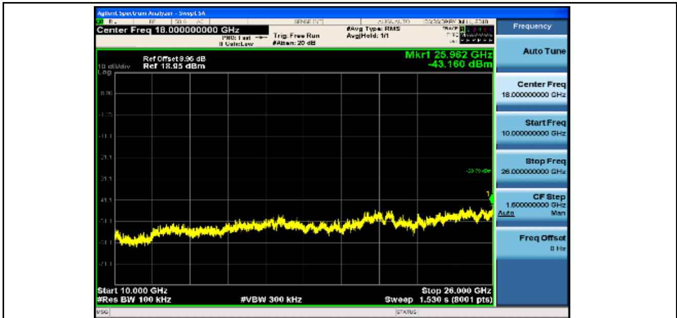
RF Conducted Spurious Emissions_11N40ISO_2422_Ant2
