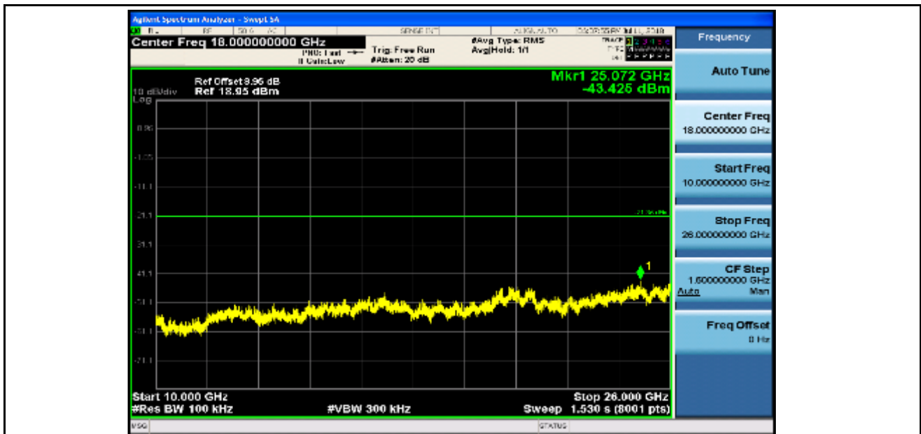
RF Conducted Spurious Emissions_11G_2412_Ant2
