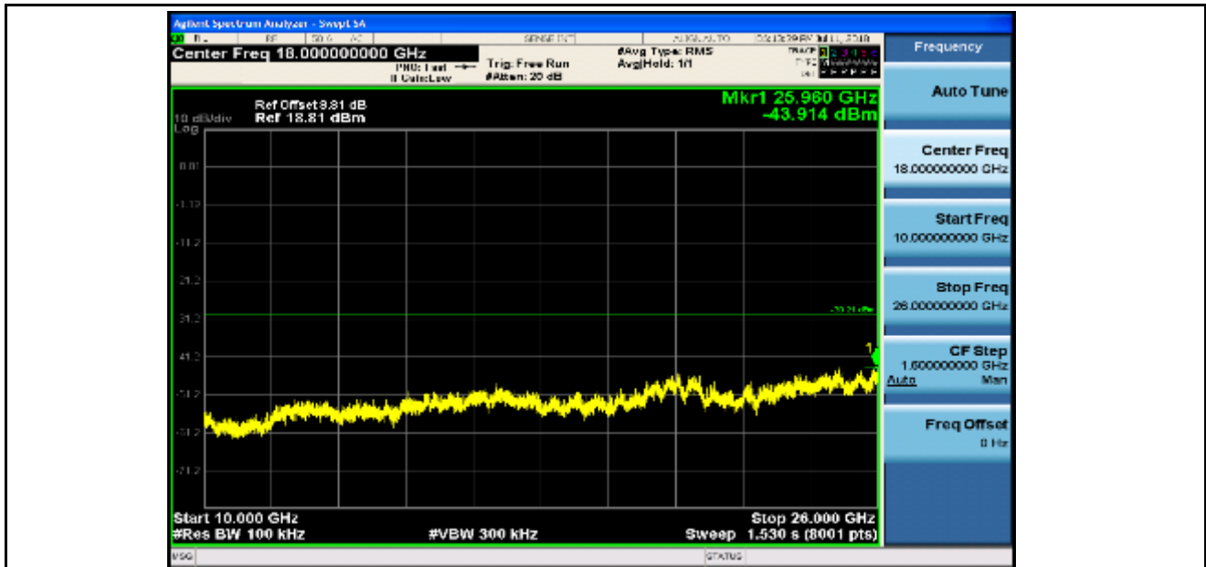
RF Conducted Spurious Emissions_11G_2437_Ant2
