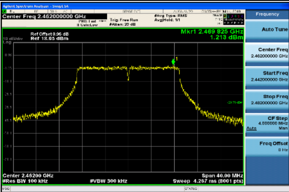
RF Conducted Spurious Emissions_11N20ISO_2462_Ant2
