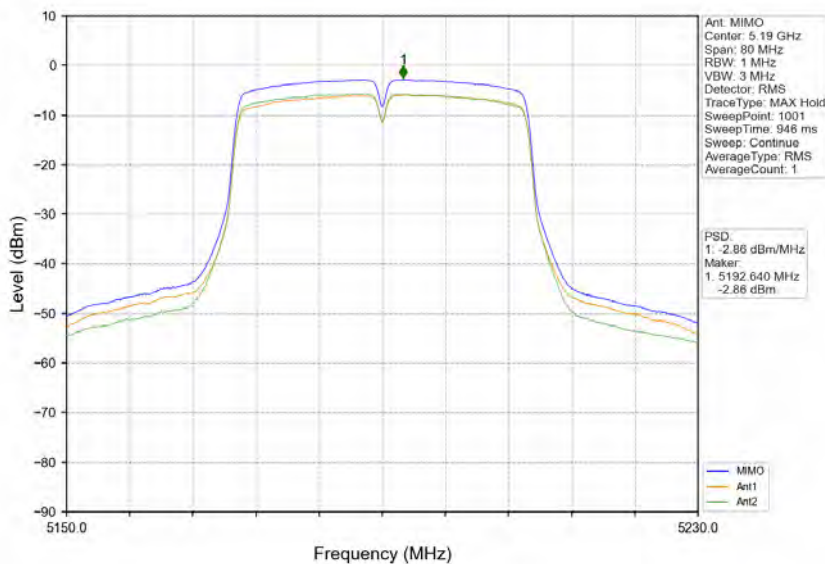
802.11n(HT40)_LCH_5190MHz_MIMO_NTNV
