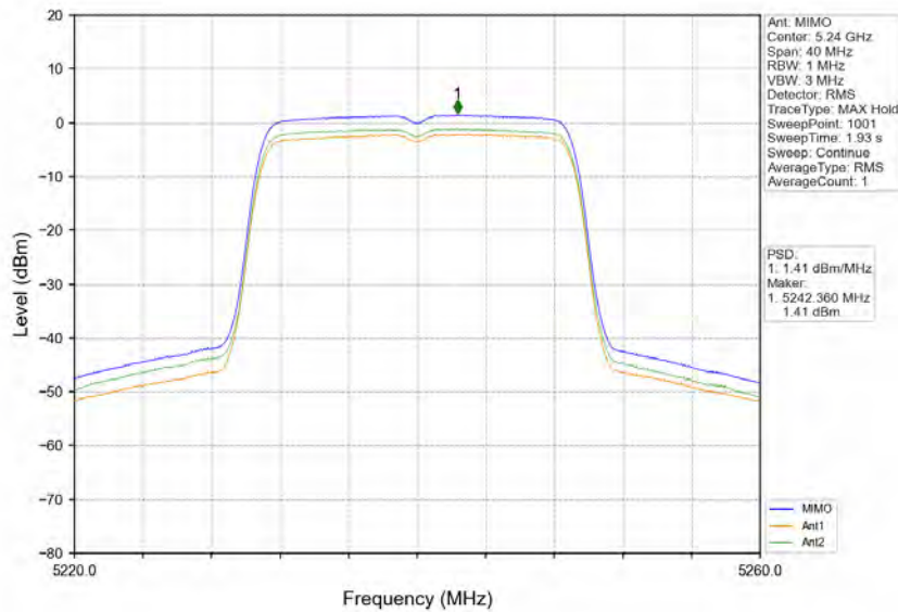
802.11ac(VHT20)_HCH_5240MHz_MIMO_NTNV
