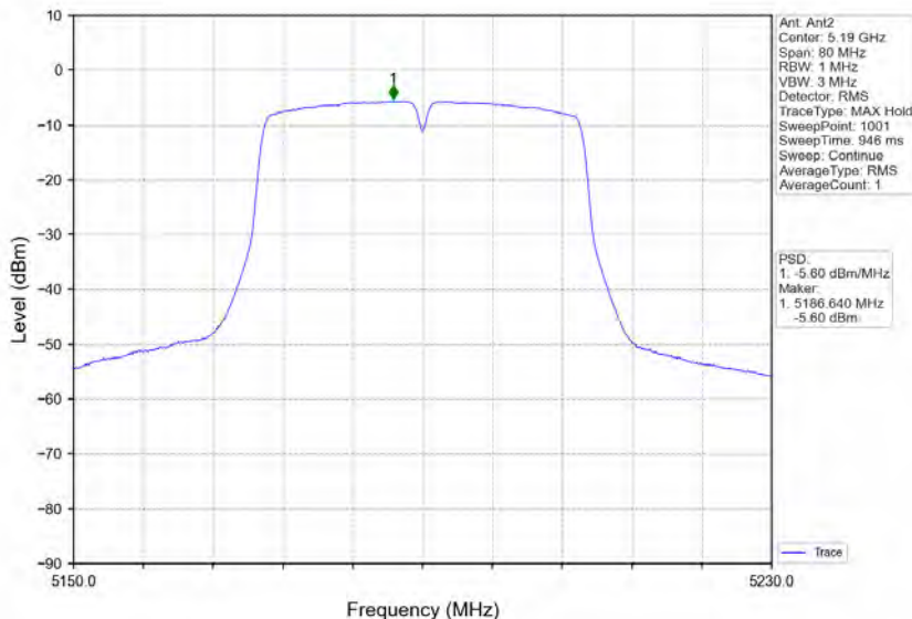
802.11n(HT40)_LCH_5190MHz_MIMO_NTNV
