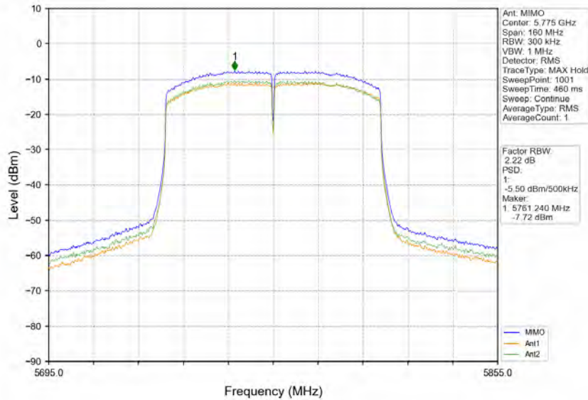
802.11ac(VHT80)_MCH_5775MHz_MIMO_NTNV
