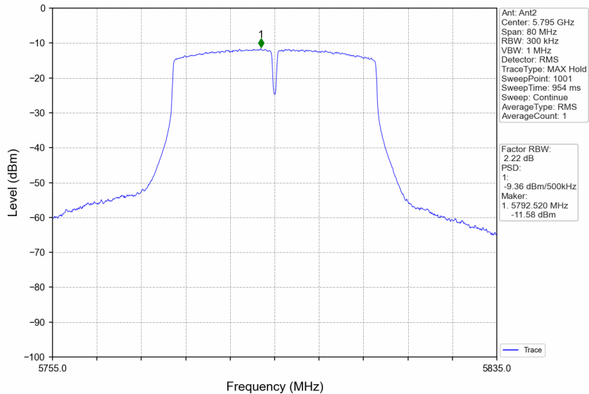
802.11ac(VHT40)_HCH_5795MHz_MIMO_NTNV
