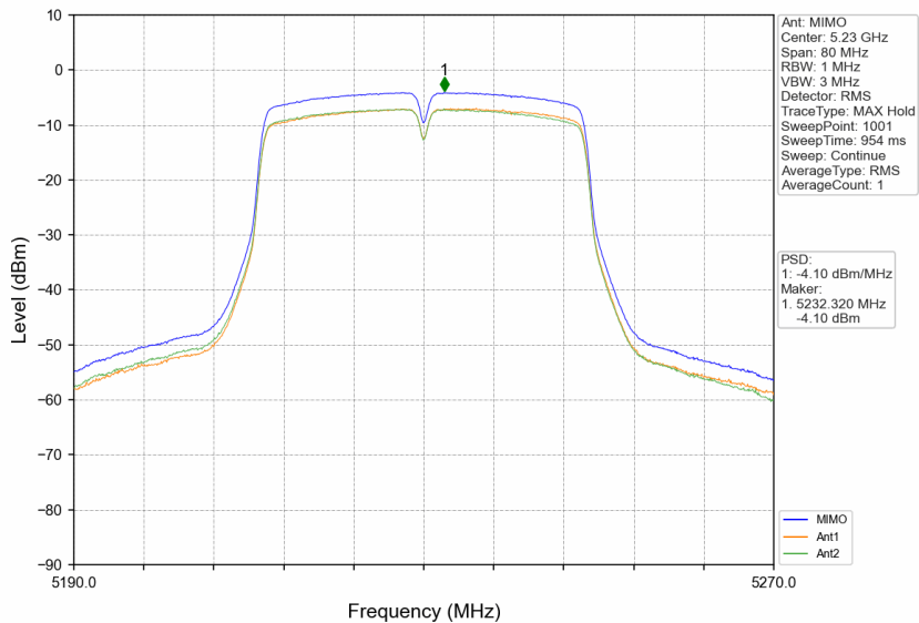
802.11ac(VHT40)_HCH_5230MHz_MIMO_NTNV
