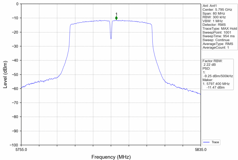
802.11ac(VHT40)_HCH_5795MHz_Ant1_NTNV
