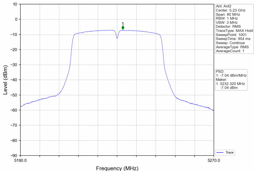
802.11ac(VHT40)_HCH_5230MHz_MIMO_NTNV
