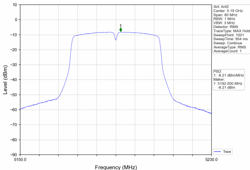
802.11ac(VHT40)_LCH_5190MHz_Ant2_NTNV
