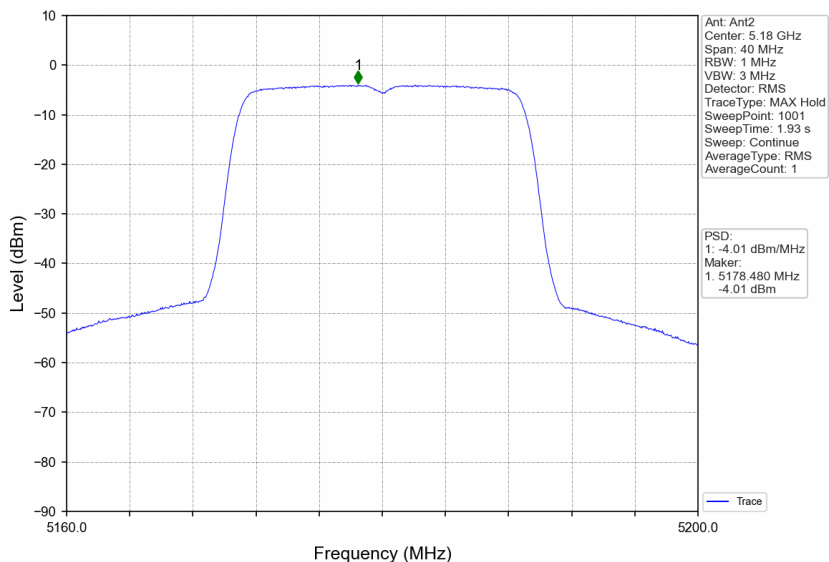
802.11ac(VHT20)_LCH_5180MHz_MIMO_NTNV
