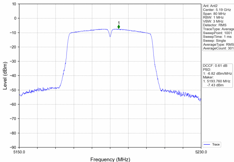
802.11n(HT40)_LCH_5190MHz_MIMO_NTNV
