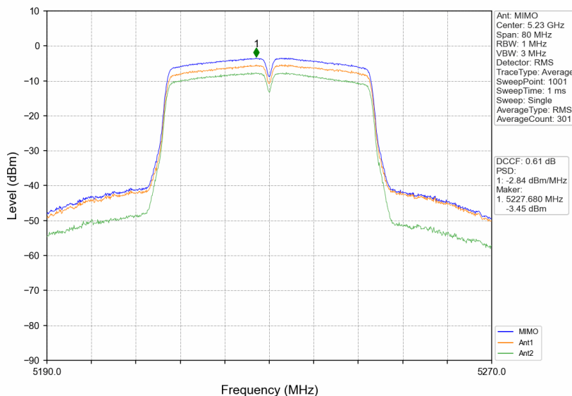
802.11ac(VHT40)_HCH_5230MHz_MIMO_NTNV
