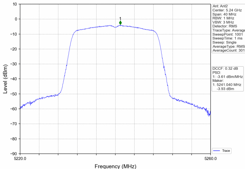
802.11ac(VHT20)_HCH_5240MHz_MIMO_NTNV
