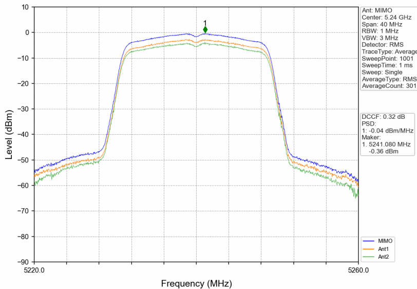
802.11ac(VHT20)_HCH_5240MHz_MIMO_NTNV
