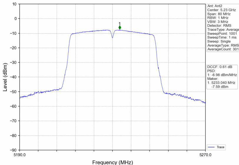
802.11ac(VHT40)_HCH_5230MHz_MIMO_NTNV
