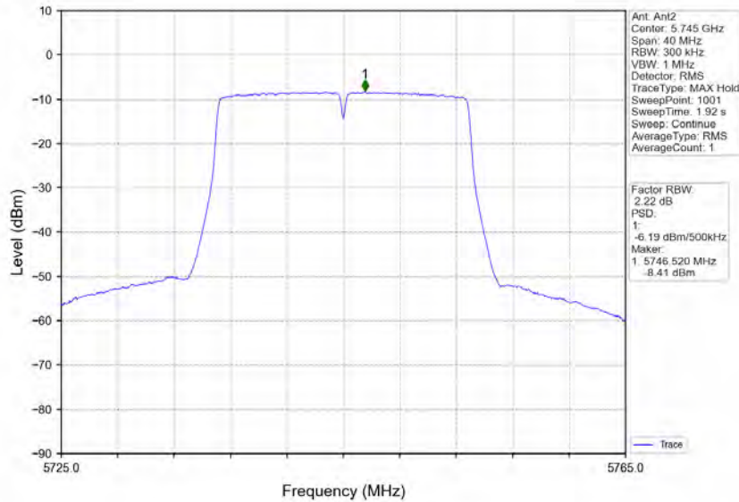
802.11ac(VHT20)_LCH_5745MHz_MIMO_NTNV
