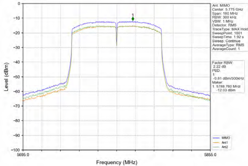
802.11ac(VHT80)_MCH_5775MHz_MIMO_NTNV
