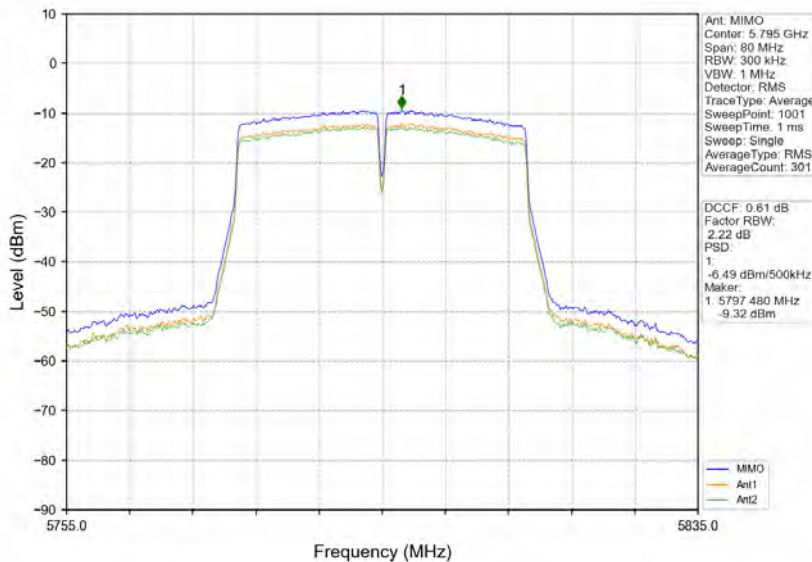
802.11ac(VHT40)_HCH_5795MHz_MIMO_NTNV
