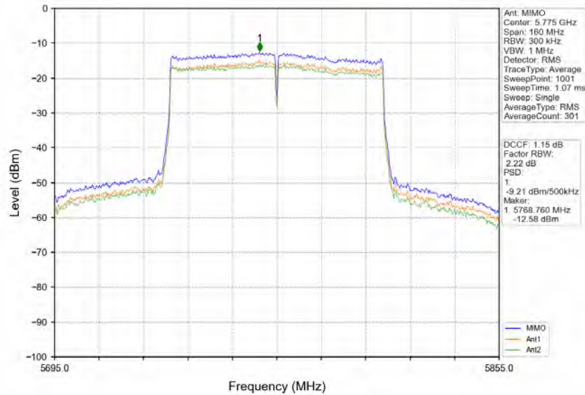
802.11ac(VHT80)_MCH_5775MHz_MIMO_NTNV
