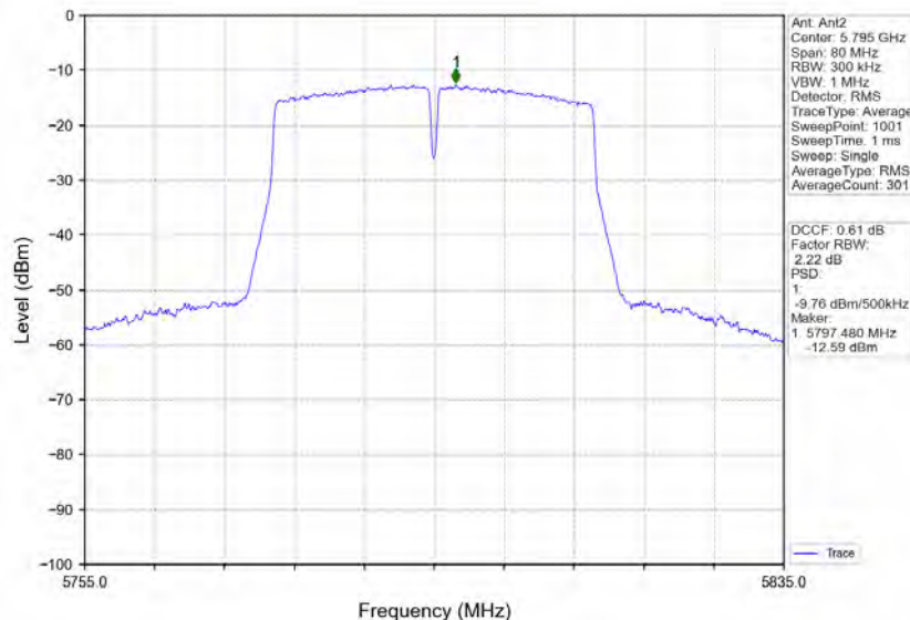
802.11ac(VHT40)_HCH_5795MHz_MIMO_NTNV
