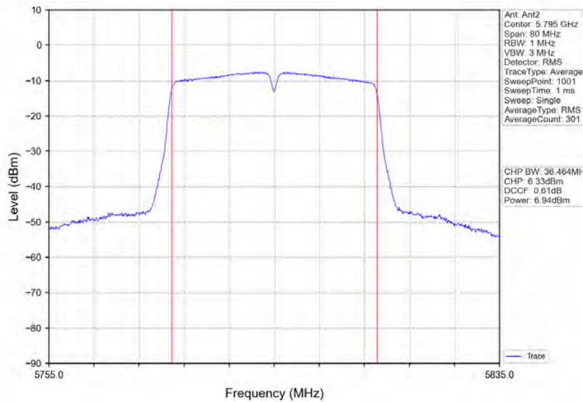
802.11ac(VHT40)_HCH_5795MHz_Ant2_NTNV
