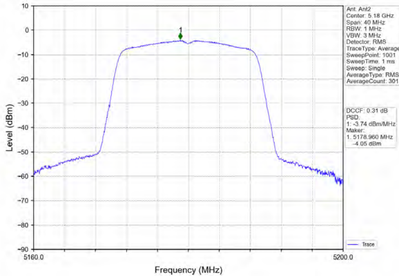
802.11ac(VHT20)_LCH_5180MHz_MIMO_NTNV
