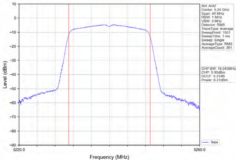
802.11ac(VHT20)_HCH_5240MHz_Ant2_NTNV
