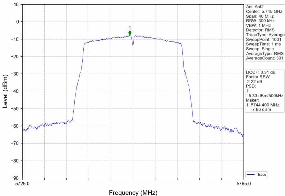
802.11ac(VHT20)_LCH_5745MHz_MIMO_NTNV
