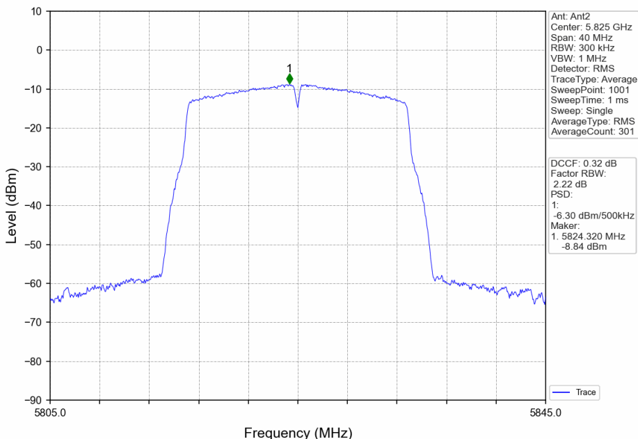
802.11ac(VHT20)_HCH_5825MHz_MIMO_NTNV
