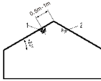
Figure 3 Mounting for gabled ceiling with slope > 20°
