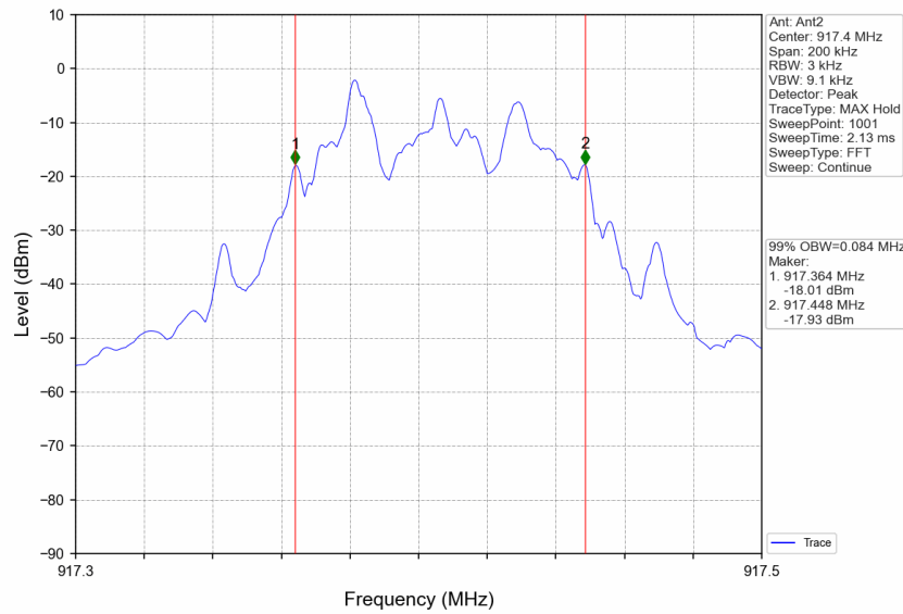
FSK_HCH_917.4MHz_Ant2_NTNV
