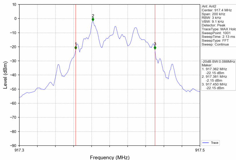
FSK_HCH_917.4MHz_Ant2_NTNV
