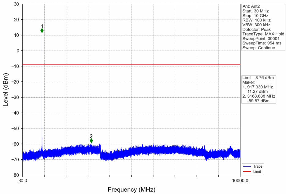
FSK_HCH_917.4MHz_Ant2_NTNV
