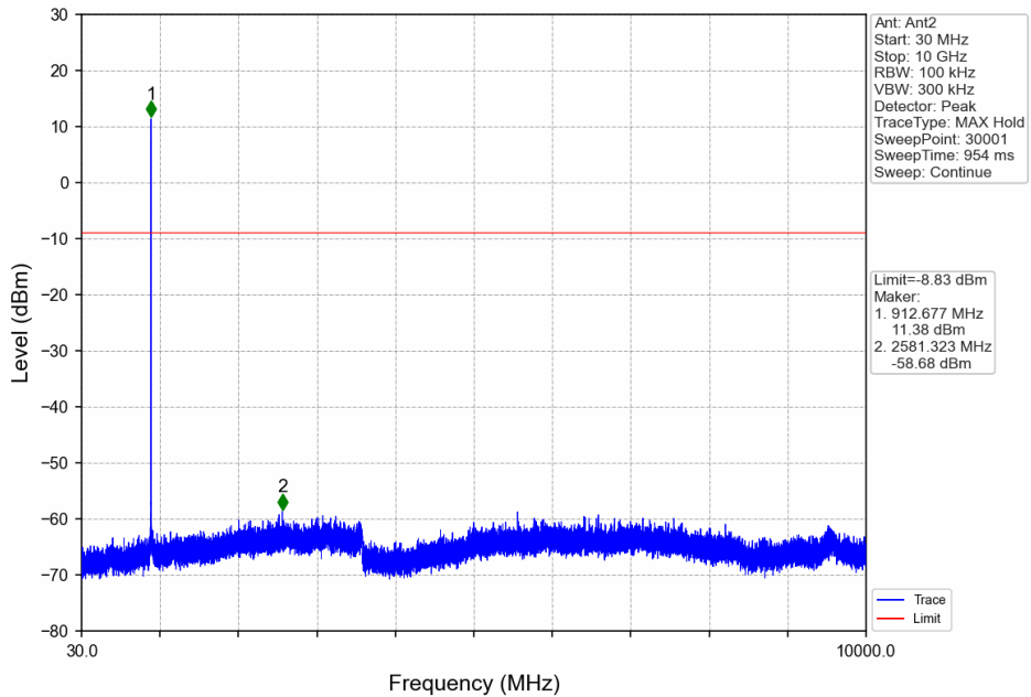
FSK_LCH_912.5MHz_Ant2_NTNV
