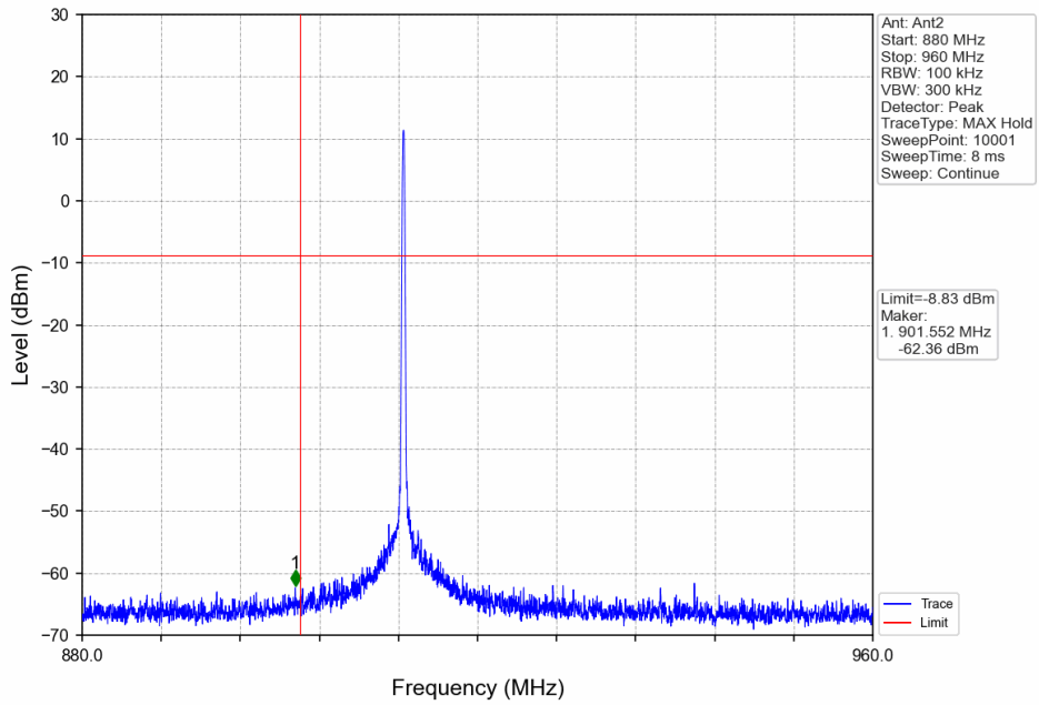
FSK_LCH_912.5MHz_Ant2_NTNV
