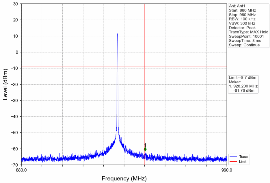
FSK_HCH_917.4MHz_Ant1_NTNV
