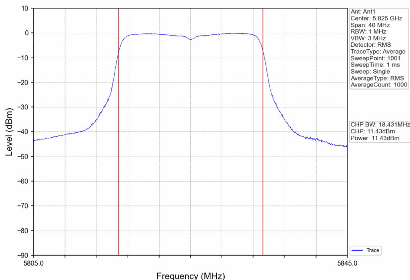
802.11ac(VHT20)_HCH_5825MHz_Ant1_NTNV
