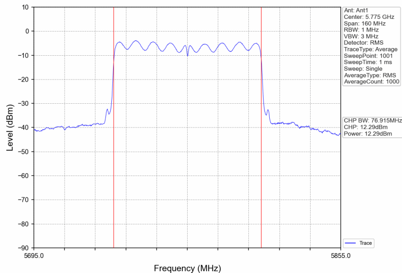
802.11ac(VHT80)_MCH_5775MHz_Ant1_NTNV
