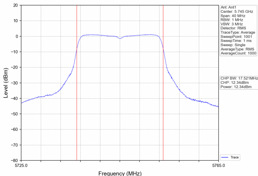
802.11a_LCH_5745MHz_Ant1_NTNV
