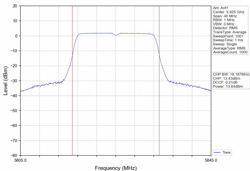
802.11a_HCH_5825MHz_Ant1_NTNV
