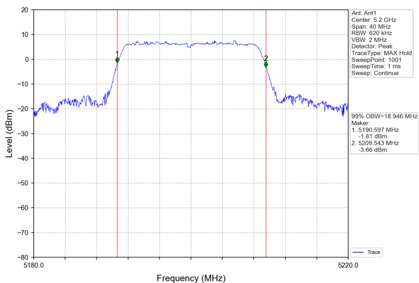
802.11n(HT20)_MCH_5200MHz_Ant1_NTNV
