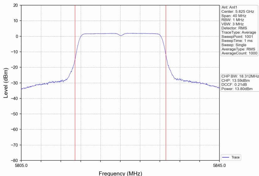
802.11a_HCH_5825MHz_Ant1_NTNV
