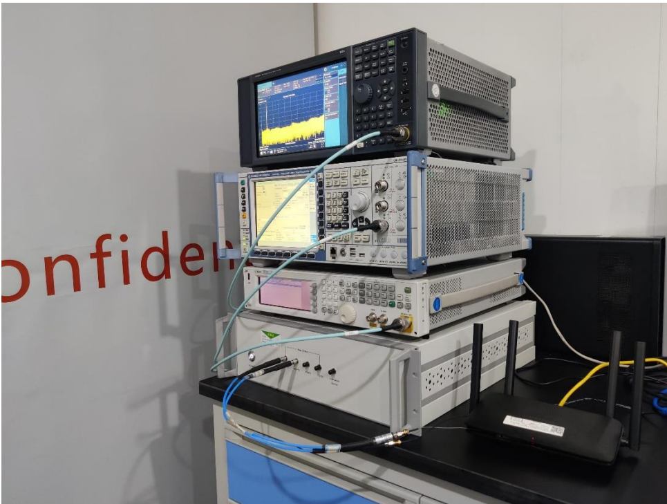
RF Conducted
