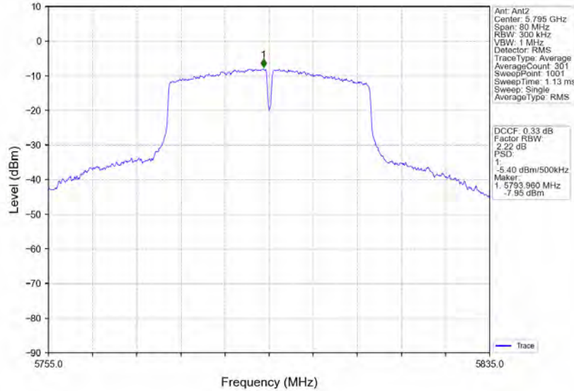
802.11ac(VHT40)_HCH_5795MHz_MIMO_NTNV
