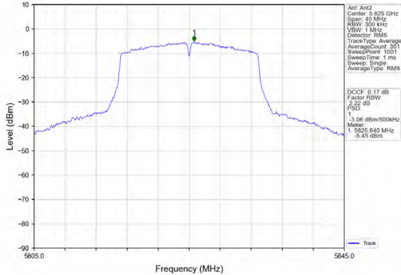
802.11ac(VHT20)_HCH_5825MHz_MIMO_NTNV
