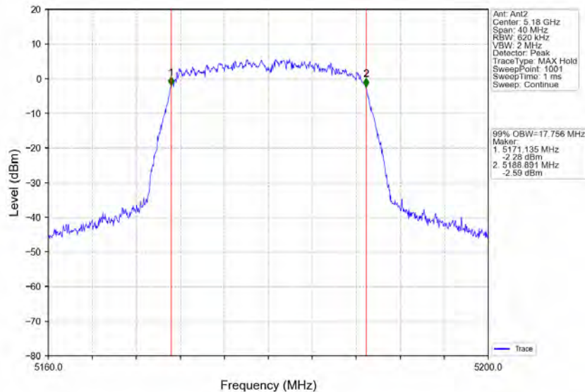
802.11ac(VHT20)_LCH_5180MHz_Ant2_NTNV
