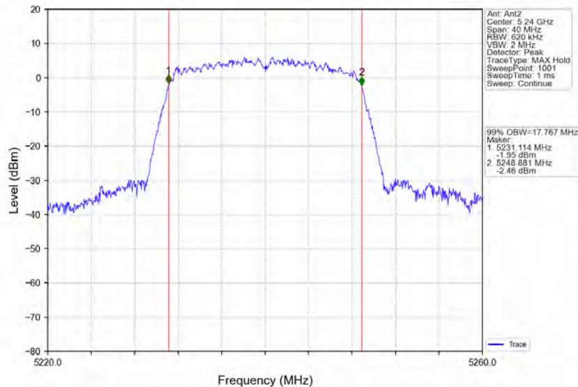
802.11ac(VHT20)_HCH_5240MHz_Ant2_NTNV
