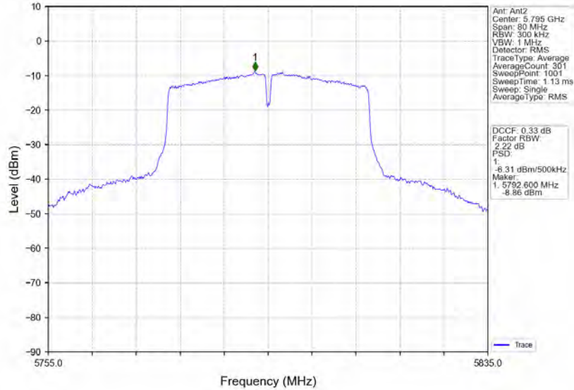
802.11ac(VHT40)_HCH_5795MHz_MIMO_NTNV
