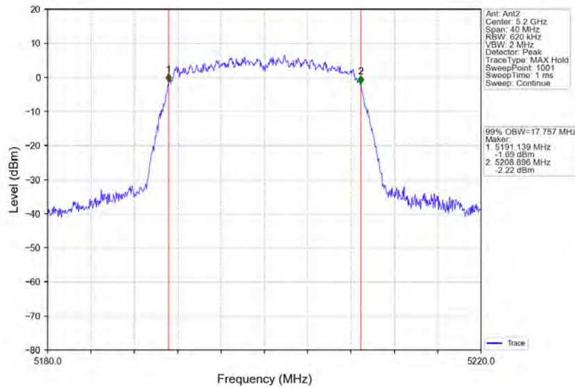
802.11ac(VHT20)_MCH_5200MHz_Ant2_NTNV
