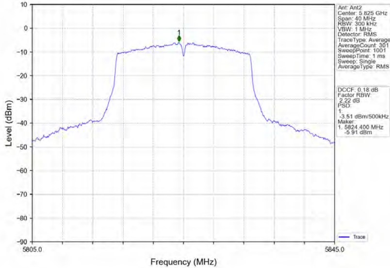
802.11ac(VHT20)_HCH_5825MHz_MIMO_NTNV
