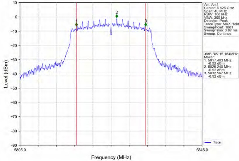
802.11ac(VHT20)_HCH_5825MHz_Ant4_NTNV
