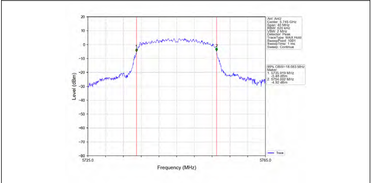
802.11n(HT20)_MCH_5785MHz_Ant3_NTNV
