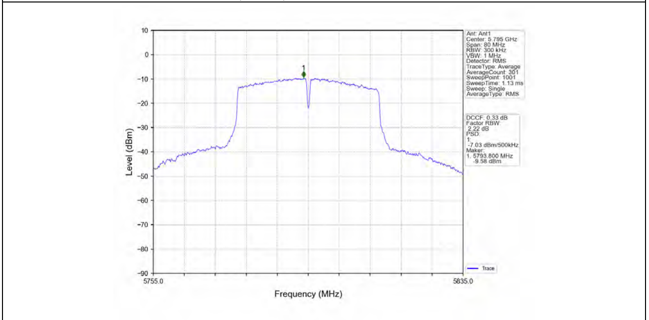
802.11ac(VHT40)_HCH_5795MHz_Ant4_NTNV
