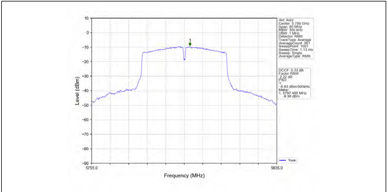
802.11ac(VHT40)_HCH_5795MHz_MIMO_NTNV
