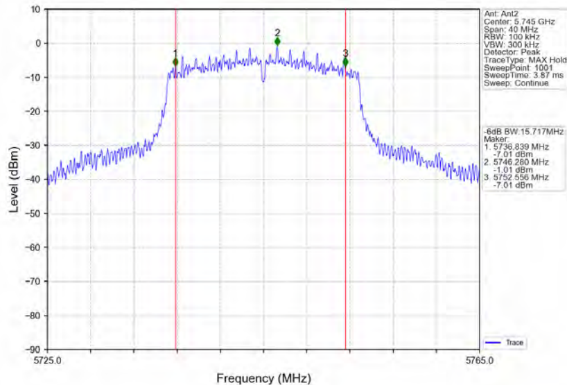
802.11ac(VHT20)_LCH_5745MHz_Ant2_NTNV
