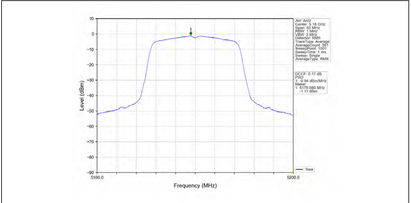
802.11ac(VHT20)_LCH_5180MHz_MIMO_NTNV
