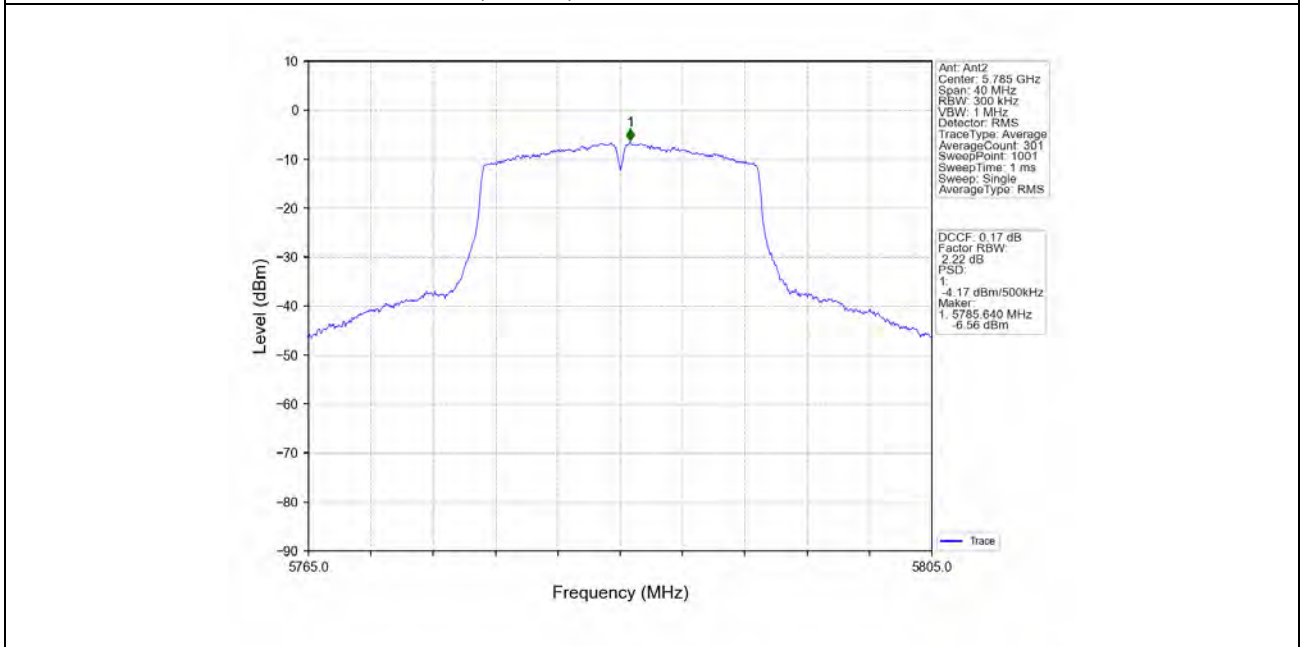
802.11ac(VHT20)_MCH_5785MHz_MIMO_NTNV
