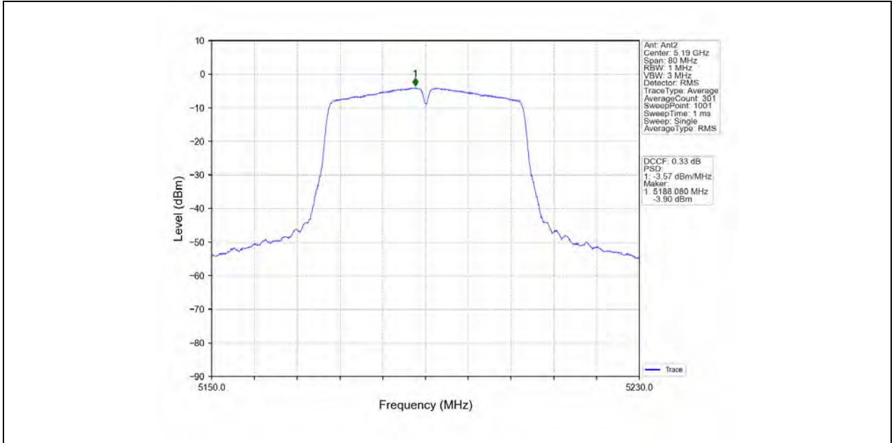
802.11n(HT40)_LCH_5190MHz_MIMO_NTNV
