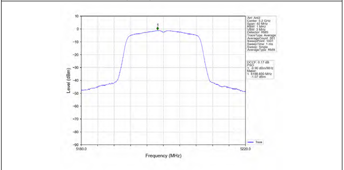
802.11ac(VHT20)_MCH_5200MHz_MIMO_NTNV
