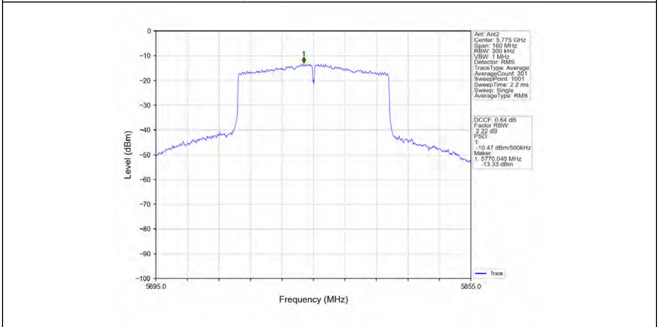
802.11ac(VHT80)_MCH_5775MHz_MIMO_NTNV
