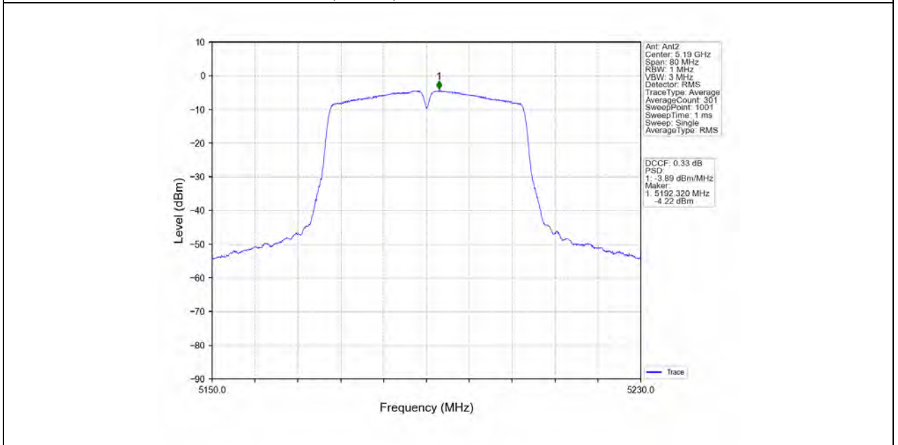
802.11ac(VHT40)_LCH_5190MHz_MIMO_NTNV
