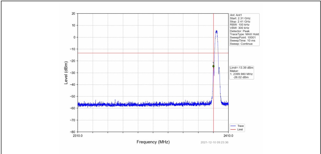
2M_LCH_2402MHz_DataRate= Ant1_NTNV
