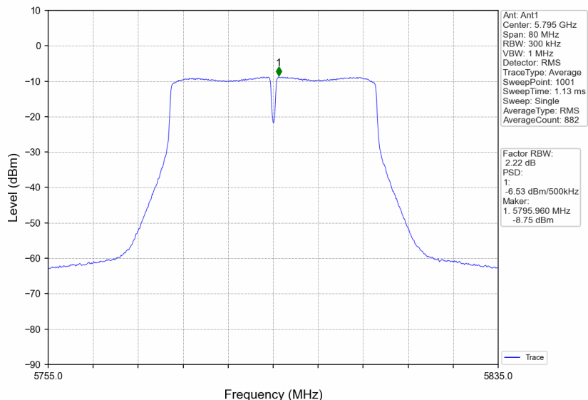
802.11ac(VHT40)_HCH_5795MHz_Ant1_NTNV
