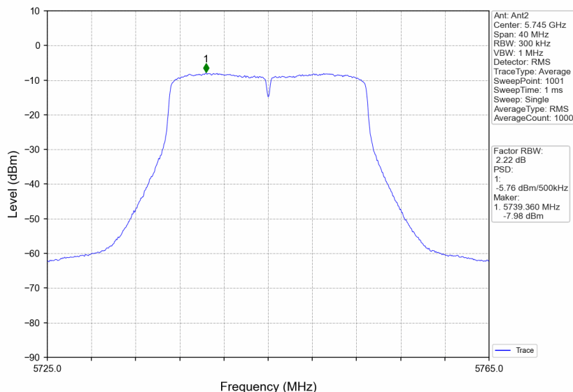
802.11ac(VHT20)_LCH_5745MHz_MIMO_NTNV
