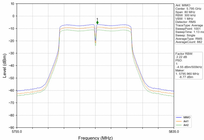
802.11ac(VHT40)_HCH_5795MHz_MIMO_NTNV
