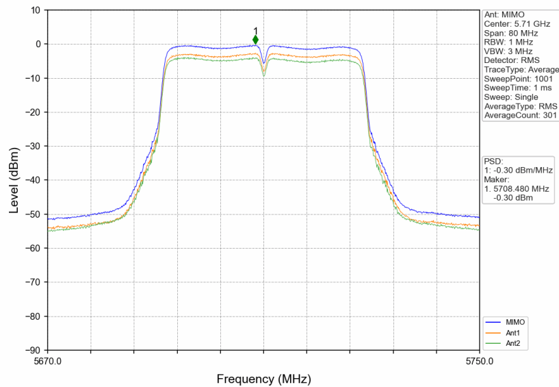
802.11ac(VHT40)_HCH_5710MHz_MIMO_NTNV
