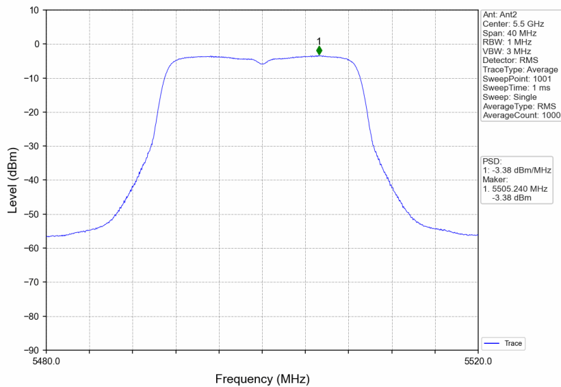
802.11ac(VHT20)_LCH_5500MHz_Ant2_NTNV
