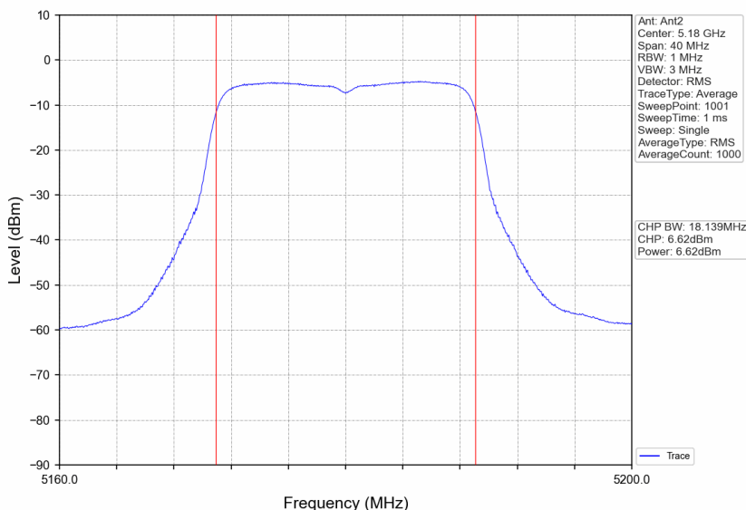
802.11ac(VHT20)_LCH_5180MHz_Ant2_NTNV
