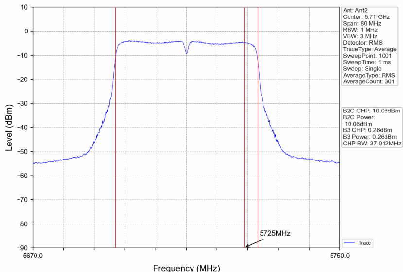
802.11n(HT40)_HCH_5710MHz_Ant2_NTNV
