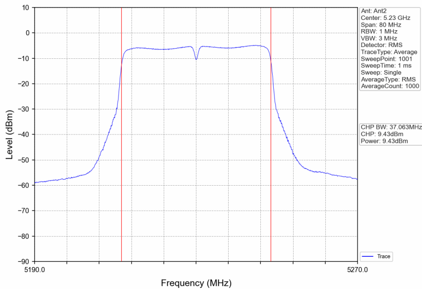
802.11ac(VHT40)_HCH_5230MHz_Ant2_NTNV
