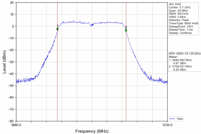
802.11ac(VHT20)_HCH_5700MHz_Ant2_NTNV
