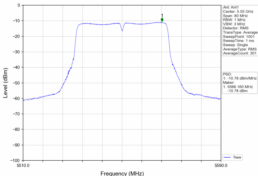
802.11n(HT40)_MCH_5550MHz_Ant1_NTNV
