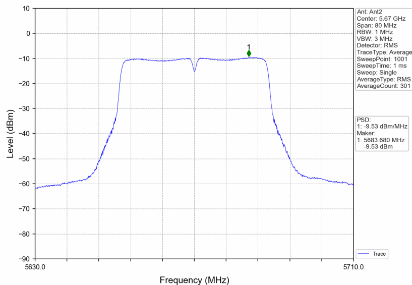
802.11n(HT40)_HCH_5670MHz_Ant2_NTNV
