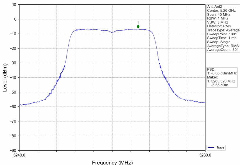
802.11ac(VHT20)_LCH_5260MHz_MIMO_NTNV
