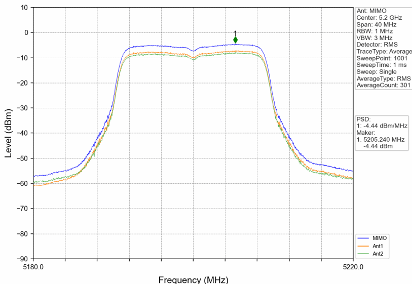
802.11ac(VHT20)_MCH_5200MHz_MIMO_NTNV
