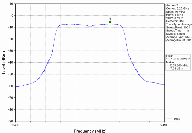
802.11n(HT20)_LCH_5260MHz_MIMO_NTNV
