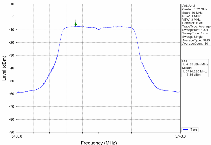
802.11ac(VHT20)_HCH_5720MHz_MIMO_NTNV
