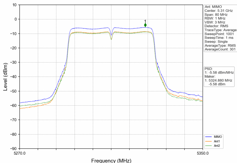
802.11n(HT40)_HCH_5310MHz_MIMO_NTNV
