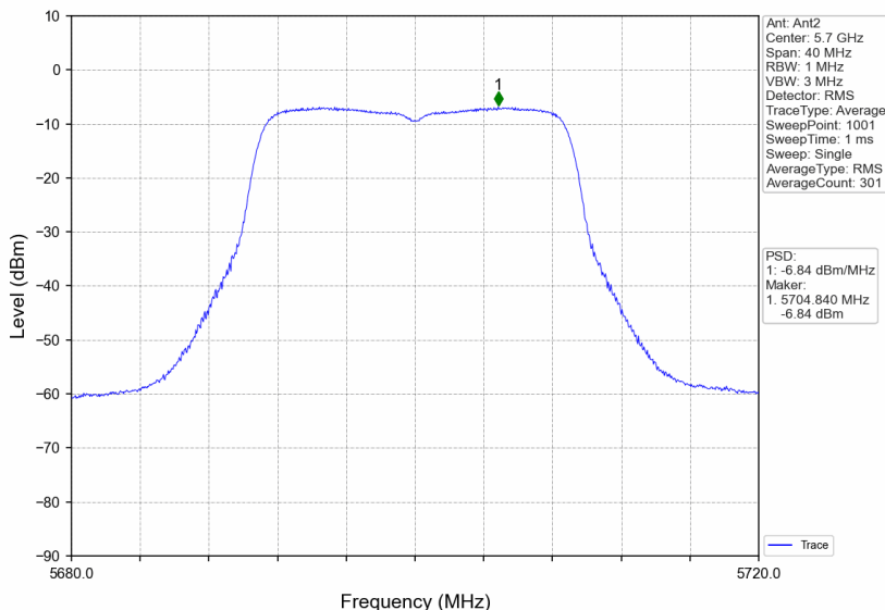
802.11ac(VHT20)_HCH_5700MHz_Ant2_NTNV
