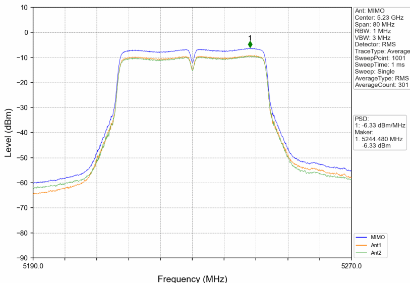
802.11n(HT40)_HCH_5230MHz_MIMO_NTNV
