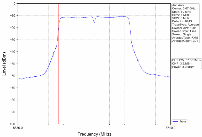
802.11ac(VHT40)_HCH_5670MHz_Ant2_NTNV
