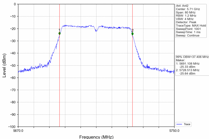
802.11ac(VHT40)_HCH_5710MHz_Ant2_NTNV
