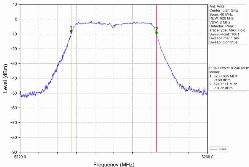
802.11ac(VHT20)_HCH_5240MHz_Ant2_NTNV
