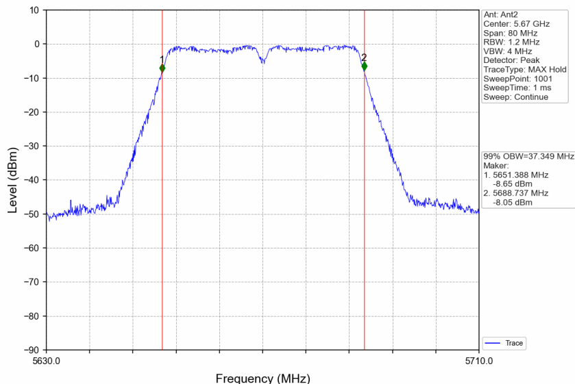
802.11n(HT40)_HCH_5670MHz_Ant2_NTNV
