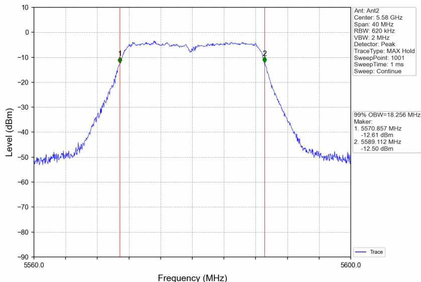
802.11ac(VHT20)_MCH_5580MHz_Ant2_NTNV
