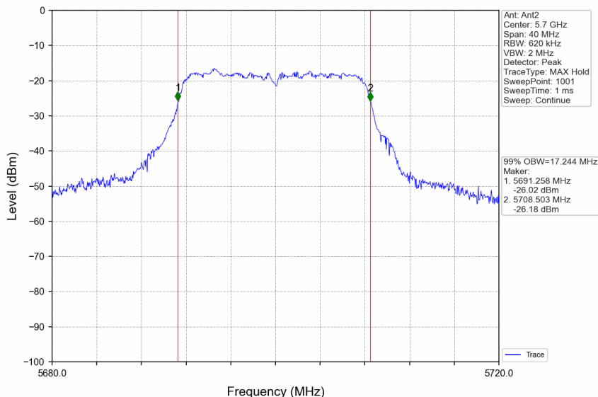
802.11ac(VHT20)_HCH_5700MHz_Ant2_NTNV
