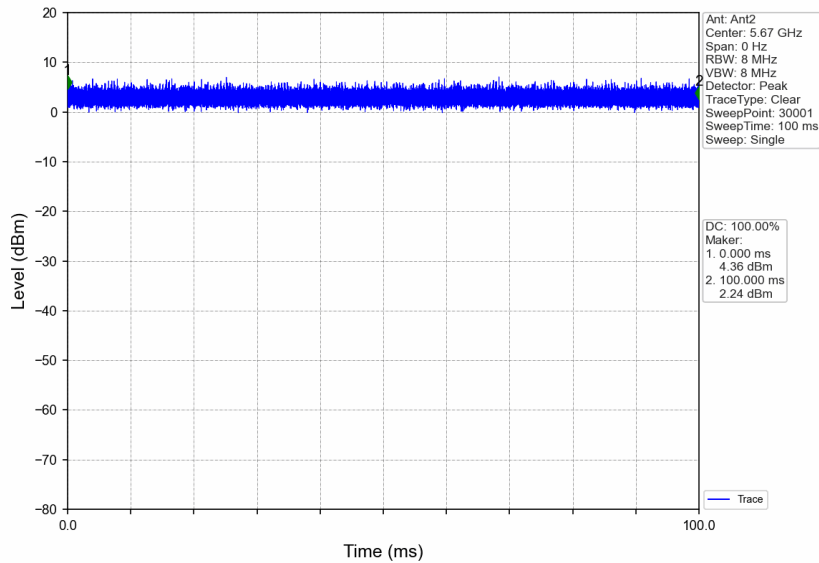
802.11ac(VHT40)_HCH_5670MHz_Ant2_NTNV
