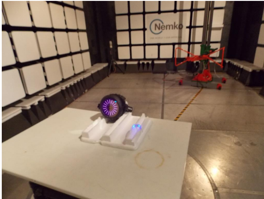
Figure 1.1-2: Radiated emissions setup photo – below 1 GHz
