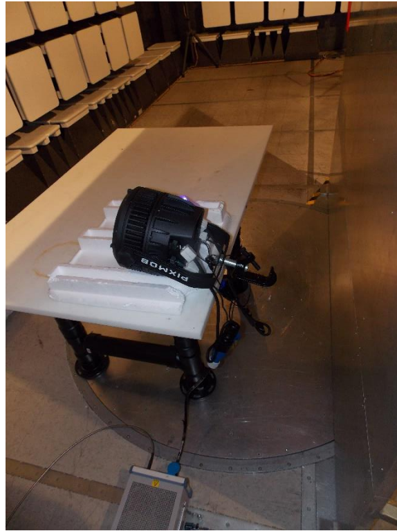
Figure 1.1-4: Conducted emissions – from AC mains power ports setup photo
