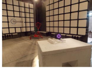
Figure 8.1-2: Radiated emissions setup photo - below 1 GHz
