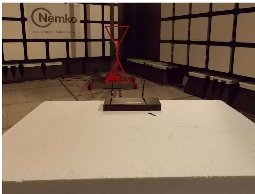
Radiated spurious (out-of-band) emissions setup photo – 30 to 1000 MHz
