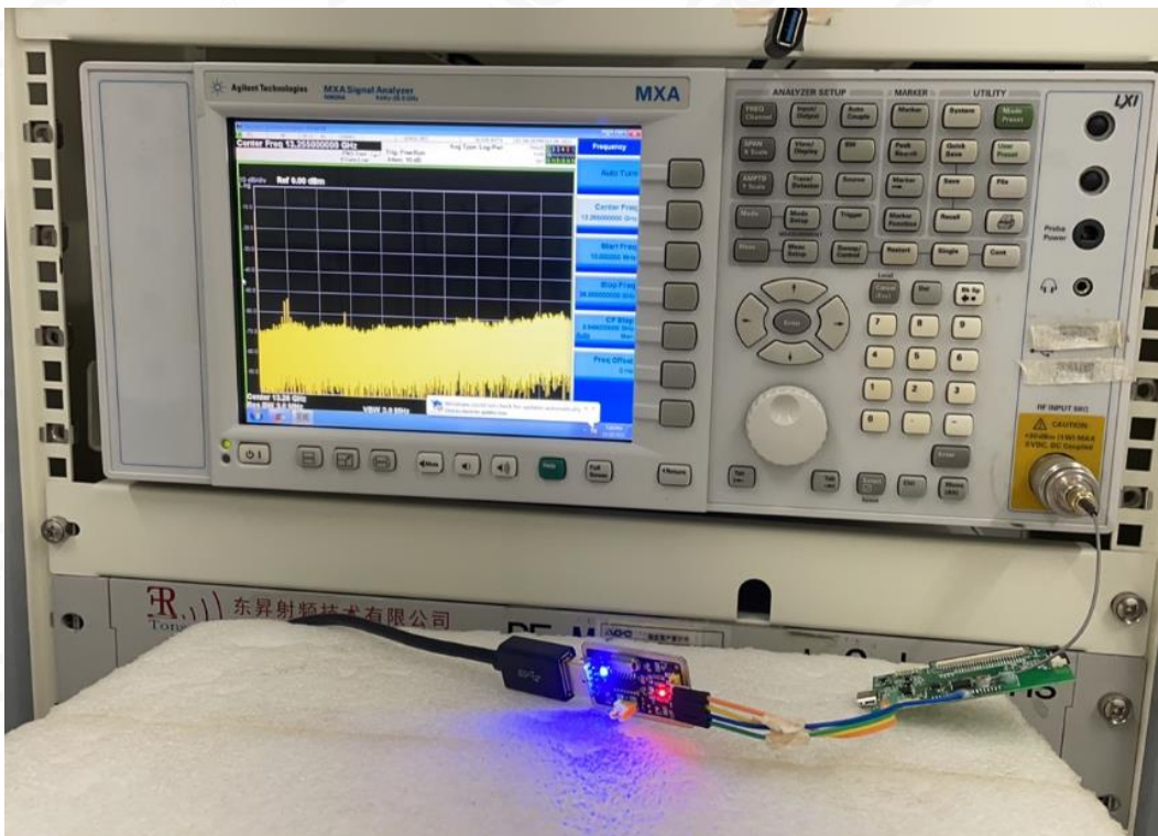
CONDUCTED TEST SETUP
