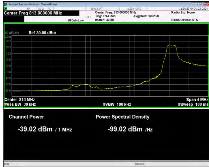
Band26(814-824) QPSK BW=1.4MHz Channel=26697 RB Size=1 Position=#0 Normal
