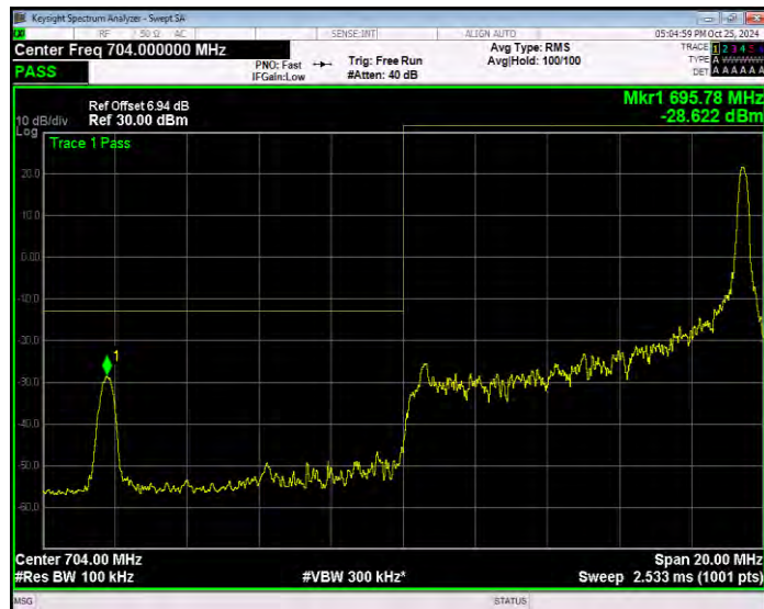
Band17 QPSK BW=10MHz Channel=23780 RB Size=50 Position=#0 Extended
