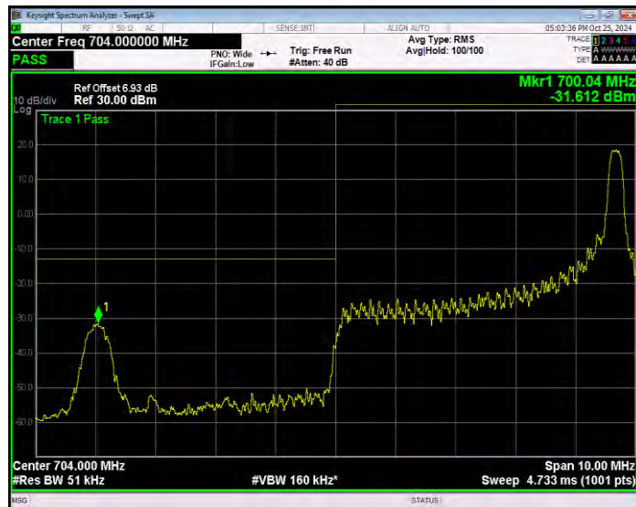
Band17 QPSK BW=5MHz Channel=23755 RB Size=25 Position=#0 Extended
