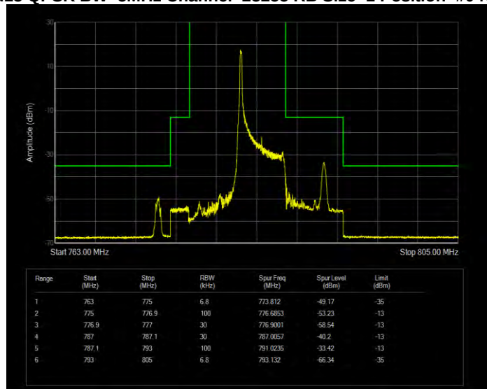
Band13 QPSK BW=5MHz Channel=23255 RB Size=1 Position=#Max Extended
