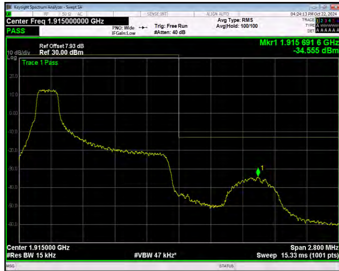
Band25 16QAM BW=1.4MHz Channel=26683 RB Size=1 Position=#Max Normal
