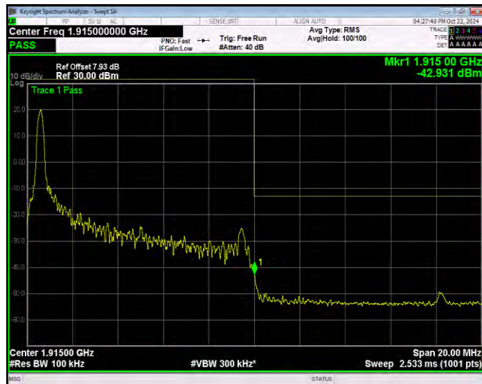
Band25 16QAM BW=10MHz Channel=26640 RB Size=1 Position=#Max Normal
