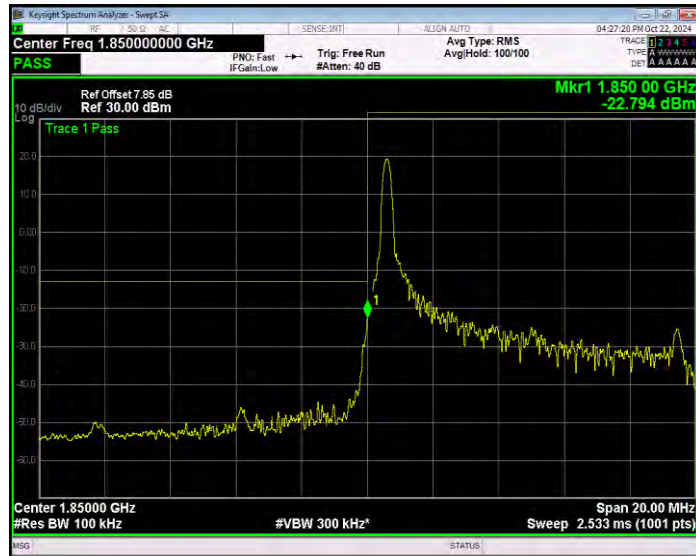
Band25 16QAM BW=10MHz Channel=26090 RB Size=1 Position=#Max Normal
