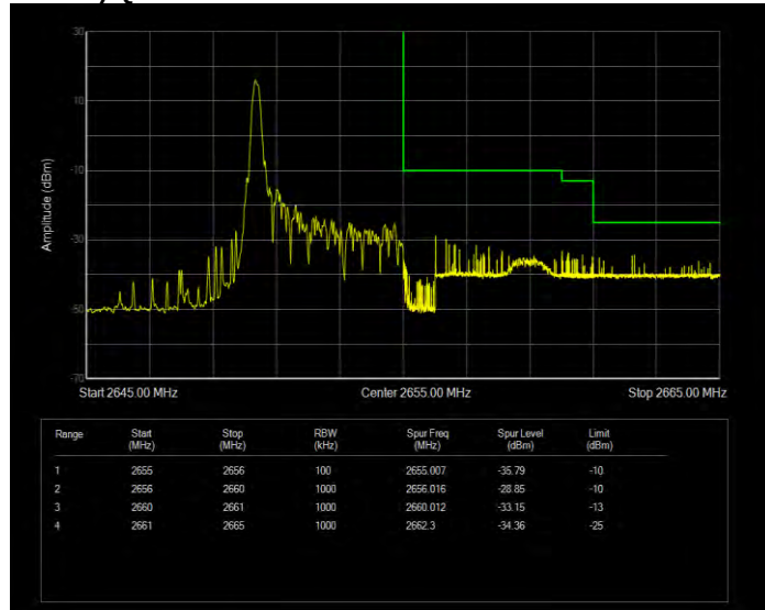
Band41(2535-2655) QPSK BW=5MHz Channel=41215 RB Size=1 Position=#Max Extended
