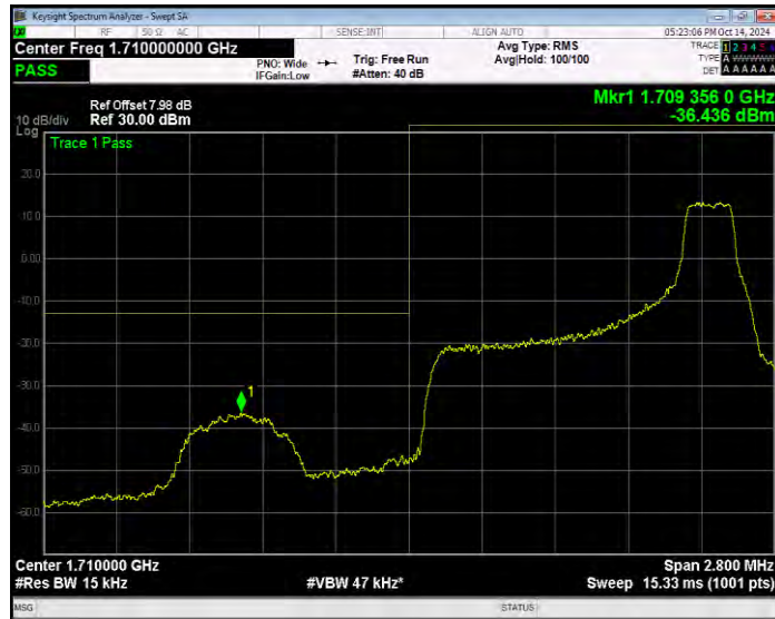
Band66 16QAM BW=1.4MHz Channel=131979 RB Size=6 Position=#0 Extended
