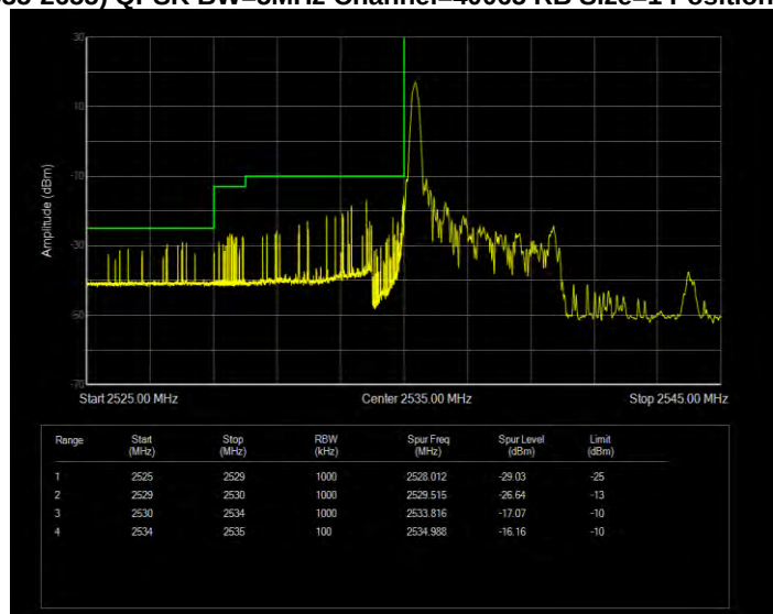
Band41(2535-2655) QPSK BW=5MHz Channel=40065 RB Size=1 Position=#Max Extended
