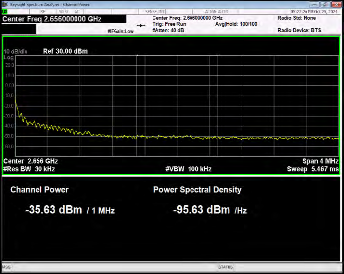
Band41(2535-2655) QPSK BW=20MHz Channel=41140 RB Size=100 Position=#0 Normal
