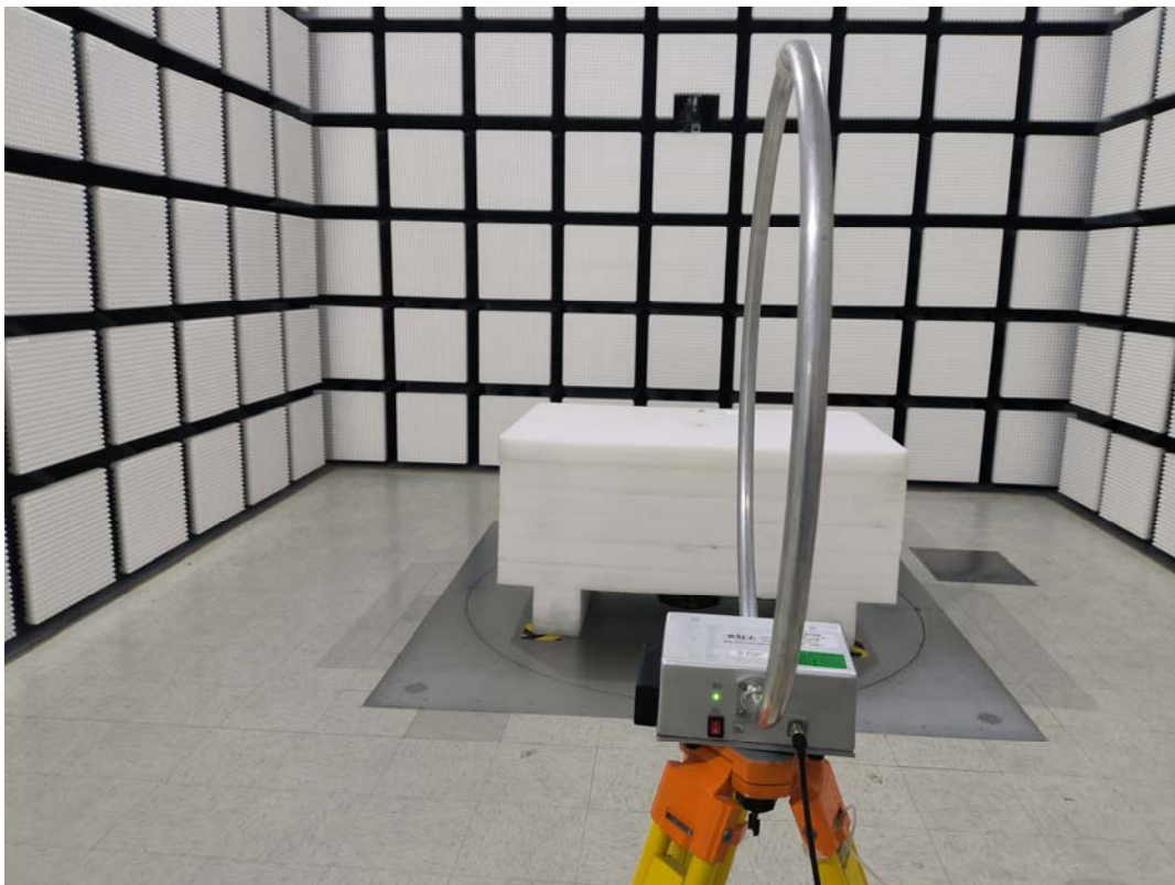
Radiated Emission 9kHz-30MHz View-Perpendicular
