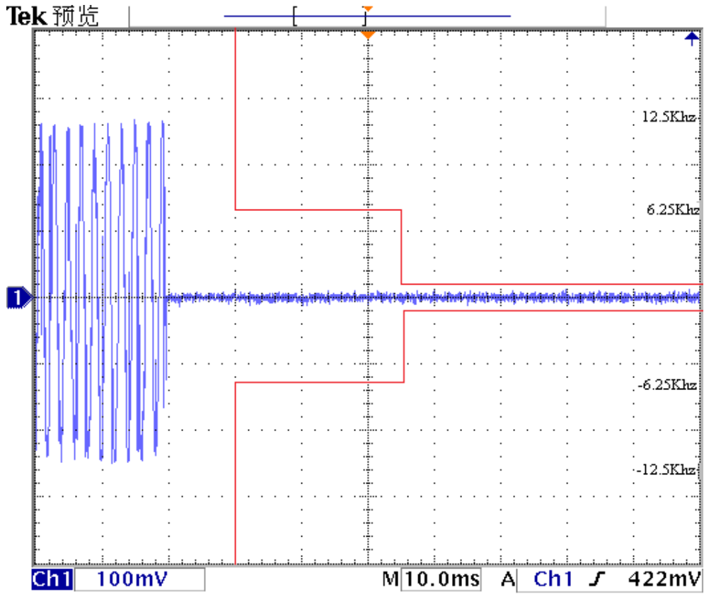
Transmitter Frequency Behavior @ 12.5 KHz Channel Separation-----On – Off
