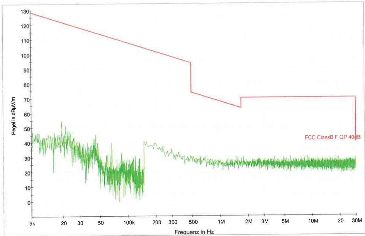
PK+_CLRWR [Stream800_CH11_OFDM_F0.Result:1] FCC ClassB F QP 40dB [..EMI radiated]
