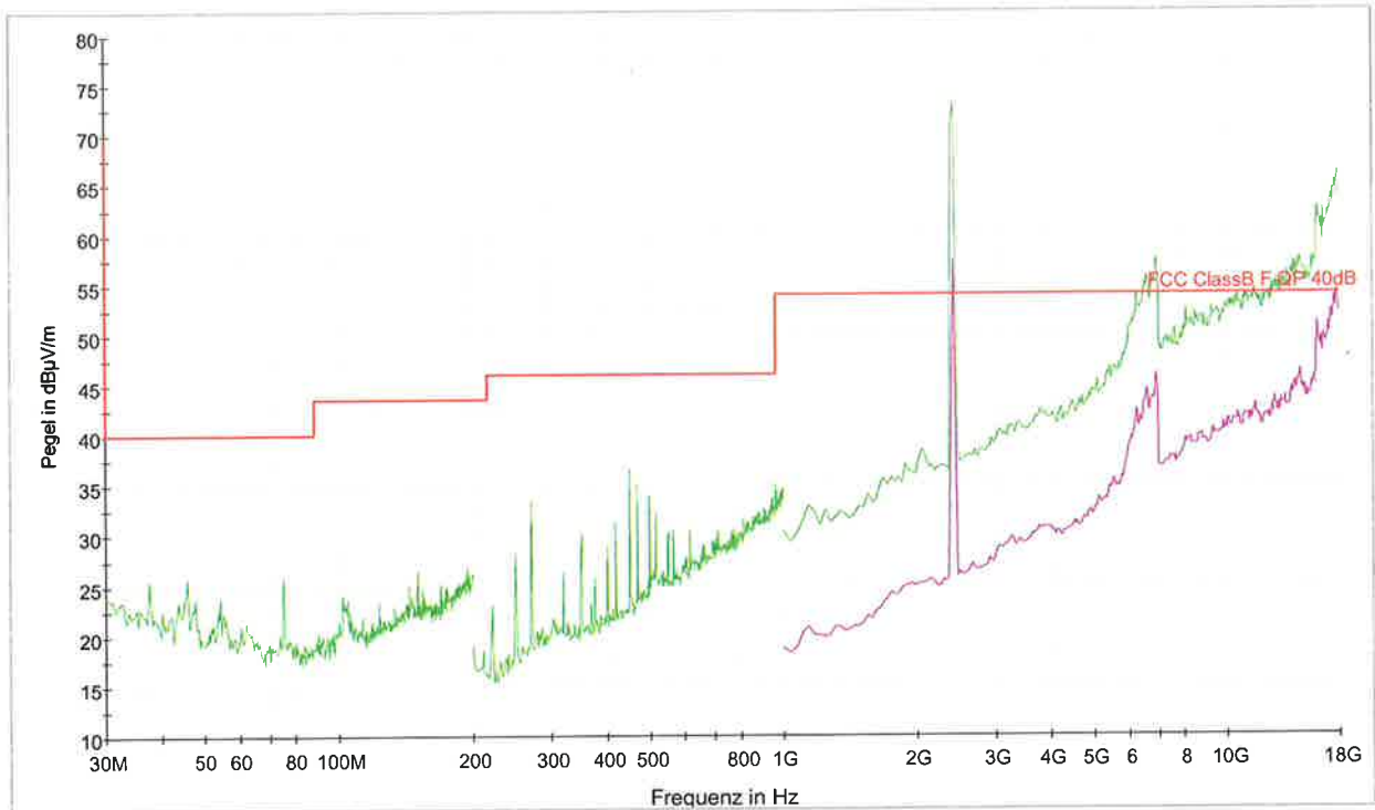
— PK+ _MAXH [Stream800_CH6_OFDM_F3.Result:2] — AVG_MAXH [Stream800_CH6_OFDM_F3.Result:4] — FCC ClassB F QP 40dB [..IEMI radiated] — PK+ _MAXH [Stream800_CH6_OFDM_F2.Result:2] — PK+ _MAXH [Stream800_CH6_OFDM_F1.Result:2]
