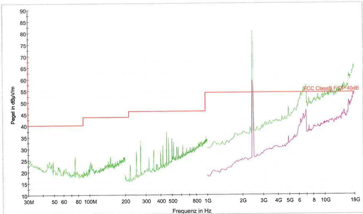
— PK+_MAXH [Stream800_CH11_DSSS_F3.Result:2] — AVG_MAXH [Stream800_CH11_DSSS_F3.Result:4] — FCC ClassB F/QP 40dB [..\EMI radiated] — PK+_MAXH [Stream800_CH11_DSSS_F1.Result:2] — PK+_MAXH [Stream800_CH11_DSSS_F2.Result:2]
