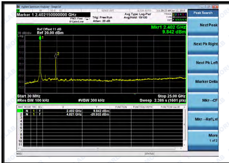
(Channel = 1, 30MHz to 25GHz)
