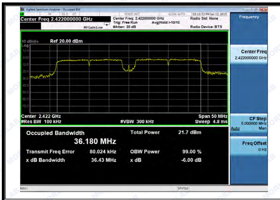
(Channel 3: 2422MHz @ 802.11n-40)
