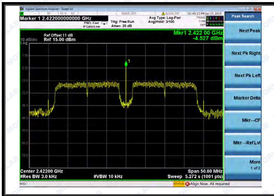
(Channel = 3 @ 802.11n-40MHz)
