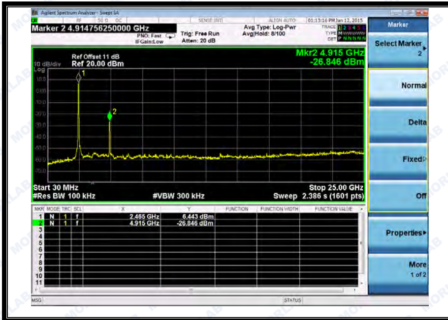
(Channel = 11, 30MHz to 25GHz)
