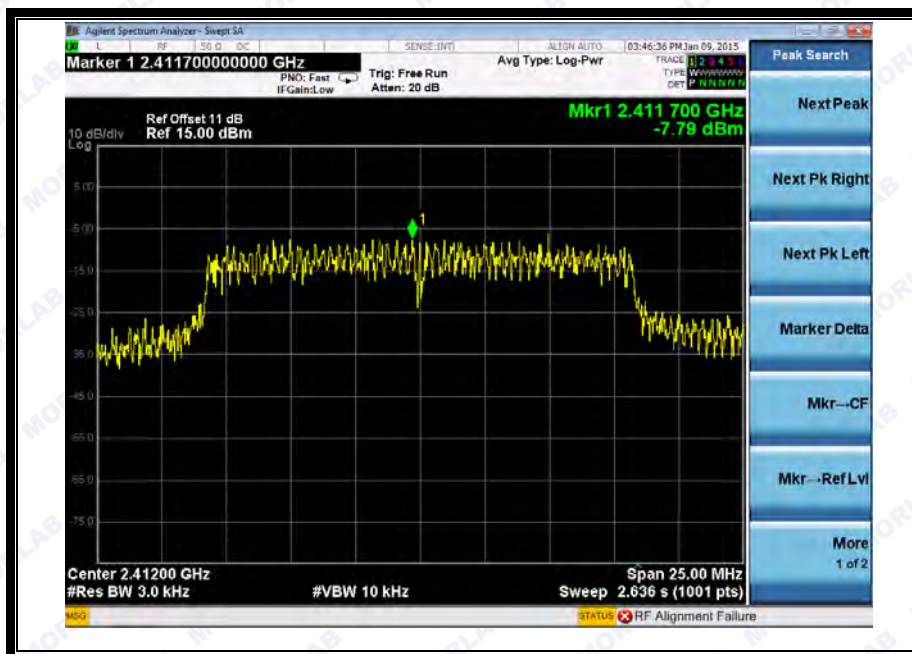
(Channel = 1 @ 802.11g)
