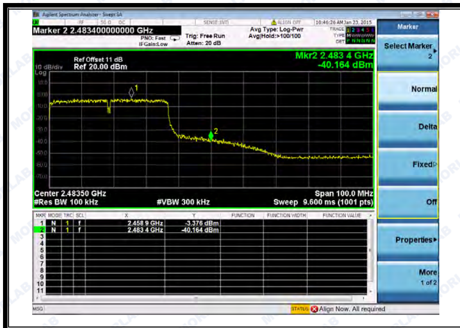
(Band Edge @ Channel = 9)
