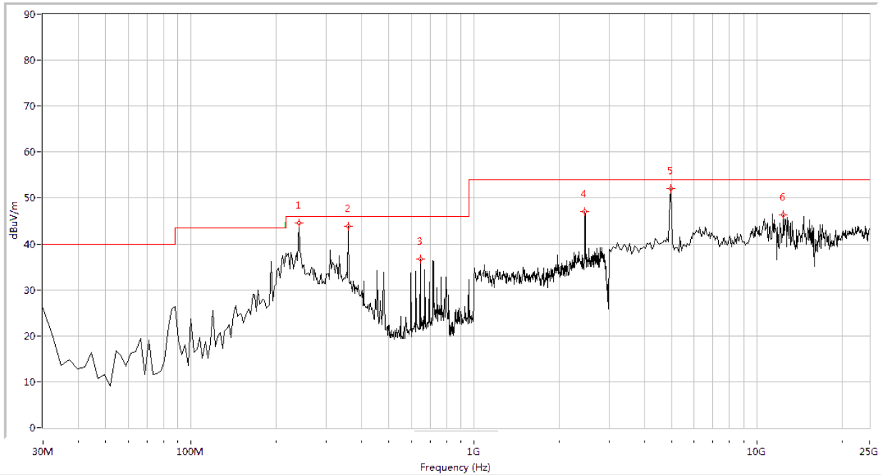
Plot for Channel = 11
