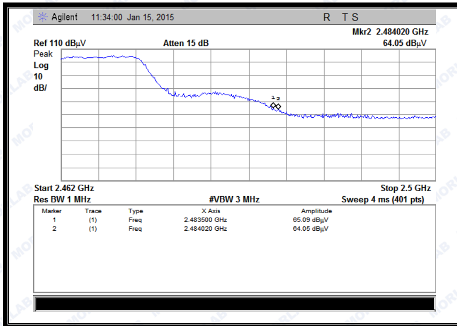
(Plot D1: Channel = 11 PEAK @ 802.11g)
