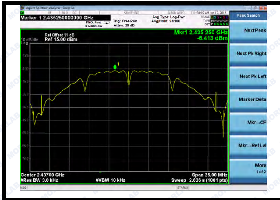
(Channel = 6 @ 802.11b)
