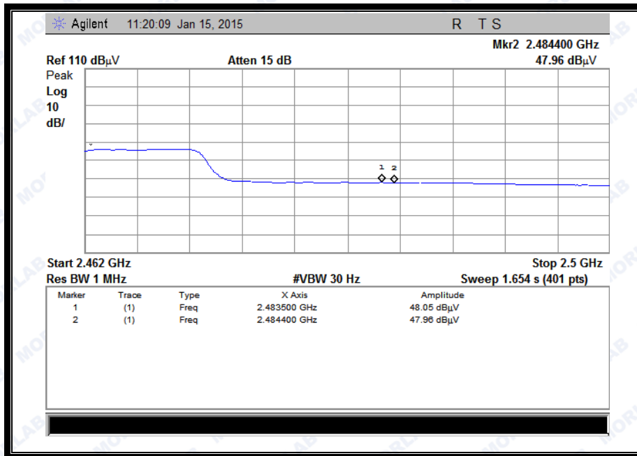
(Plot F2: Channel = 9 AVG @ 802.11n-40)
