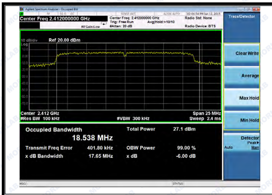
(Channel 1: 2412MHz @ 802.11n-20)
