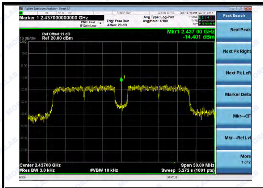
(Channel = 6 @ 802.11n-40MHz)
