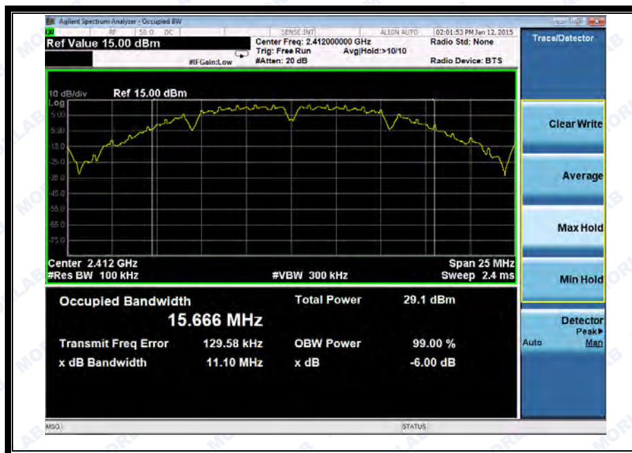
(Channel 1: 2412MHz @ 802.11b)
