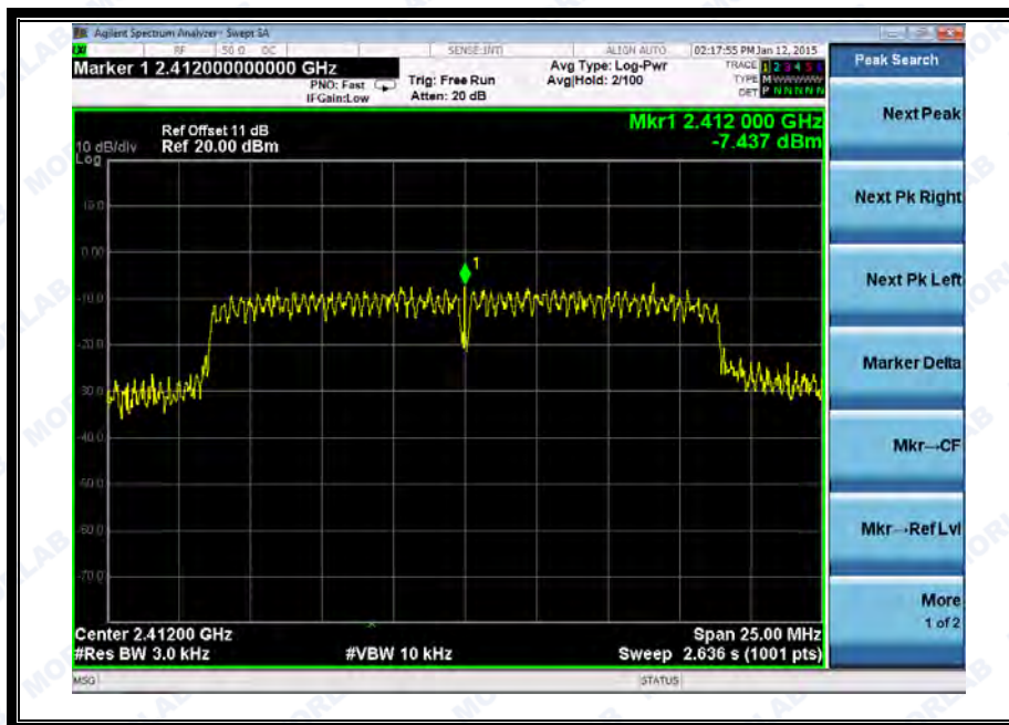
(Channel = 1 @ 802.11n-20MHz)
