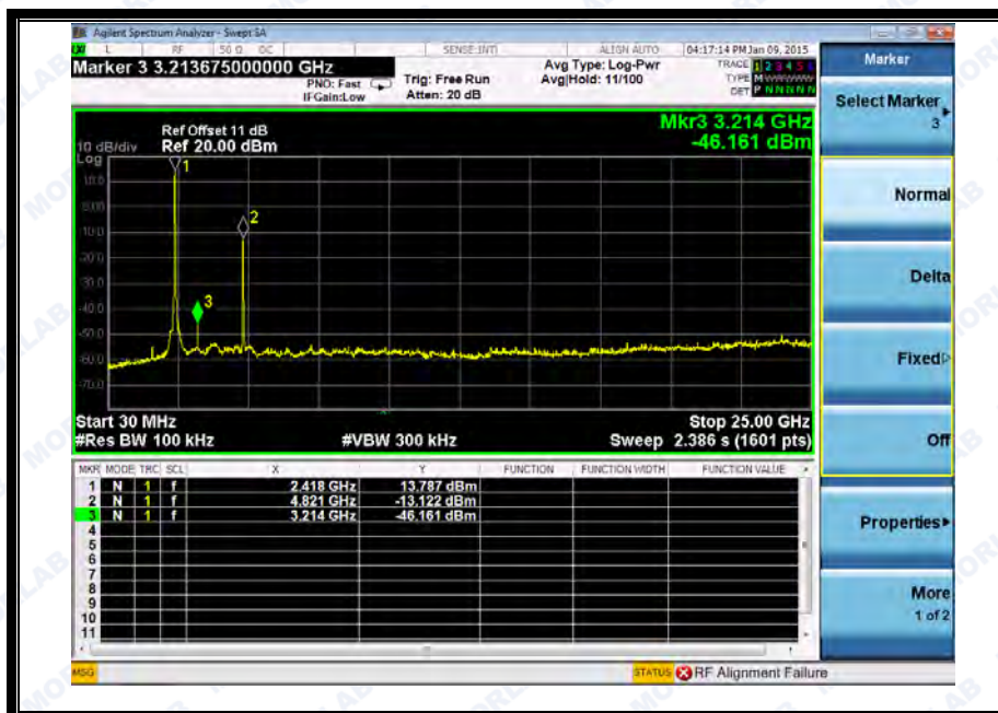
(Channel = 1, 30MHz to 25GHz)
