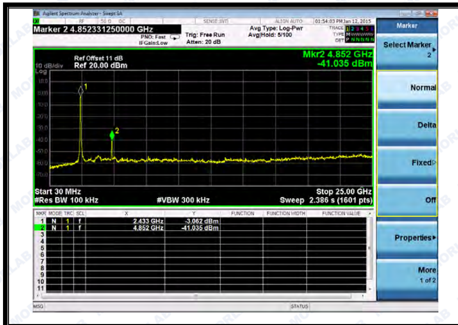
(Channel = 3, 30MHz to 25GHz)
