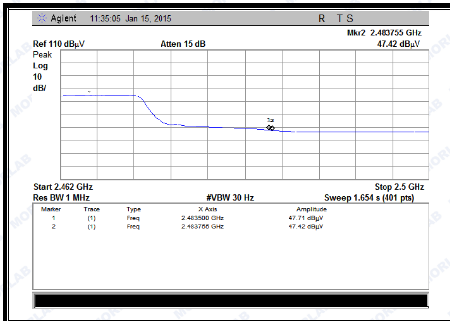
(Plot D2: Channel = 11 AVG @ 802.11g)
