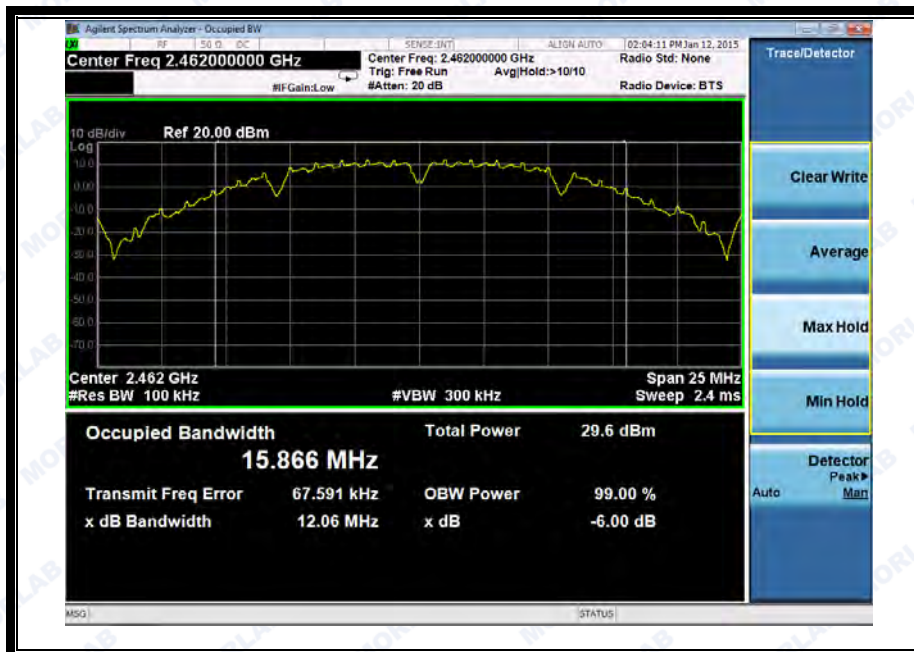
(Channel 11: 2462MHz @ 802.11b)
