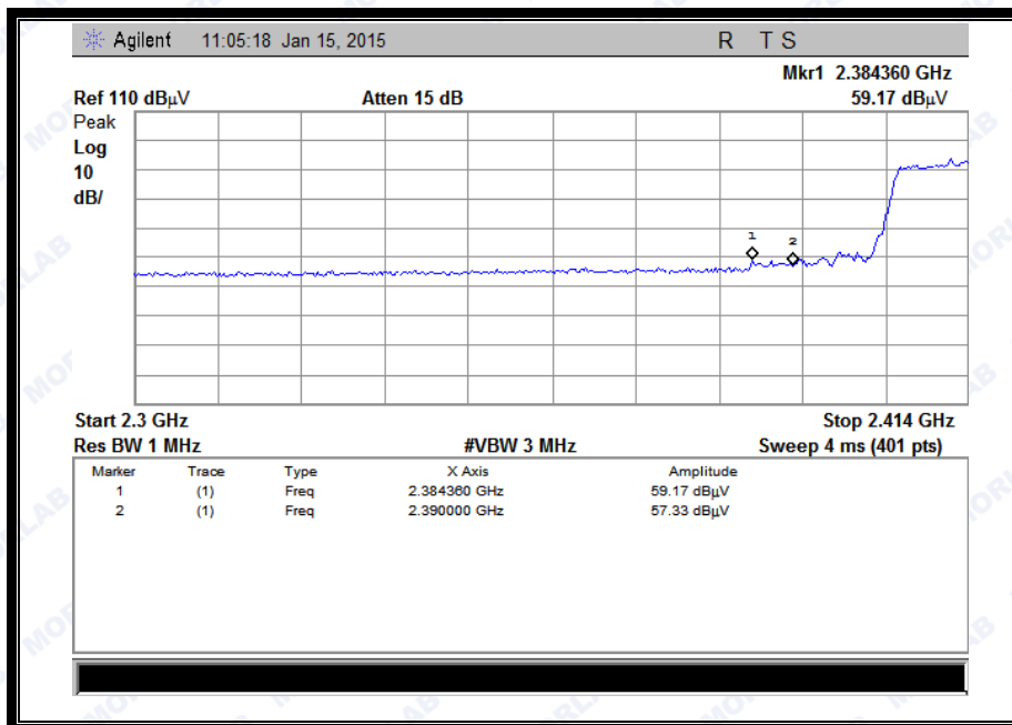
(Plot E1: Channel = 3 PEAK @ 802.11n-40)
