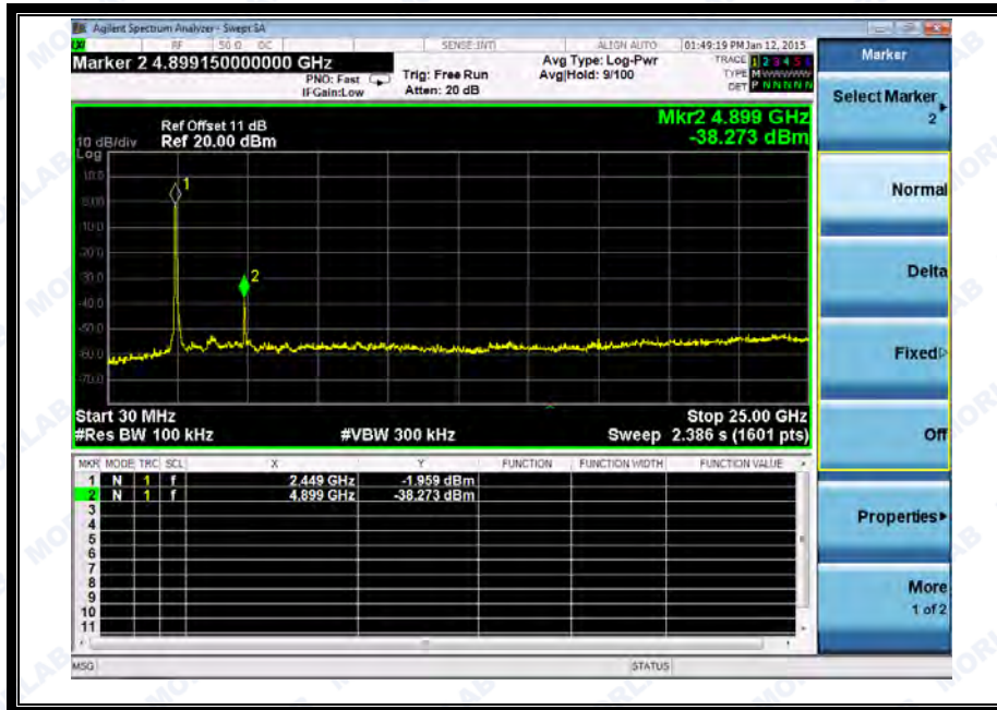
(Channel = 9, 30MHz to 25GHz)
