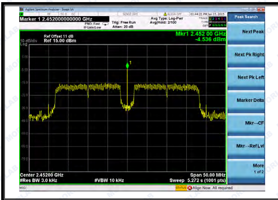
(Channel = 9 @ 802.11n-40MHz)
