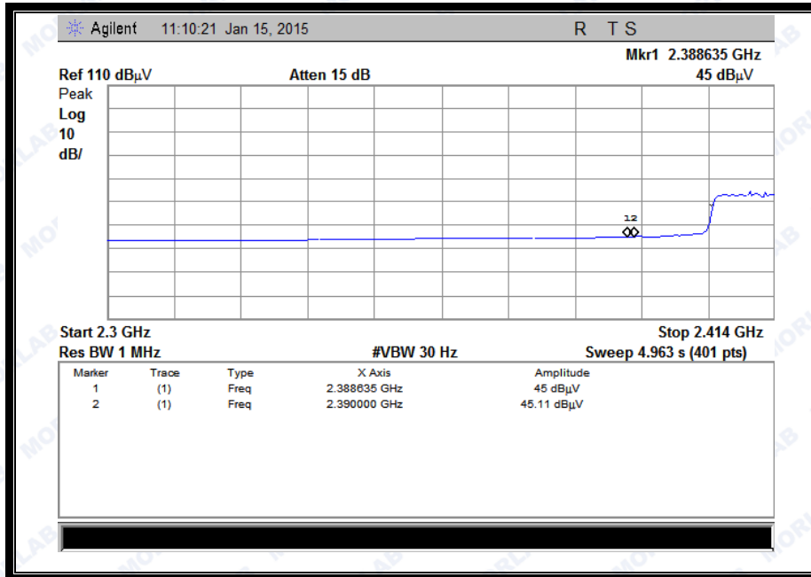
(Plot E2: Channel = 3 AVG @ 802.11n-40)
