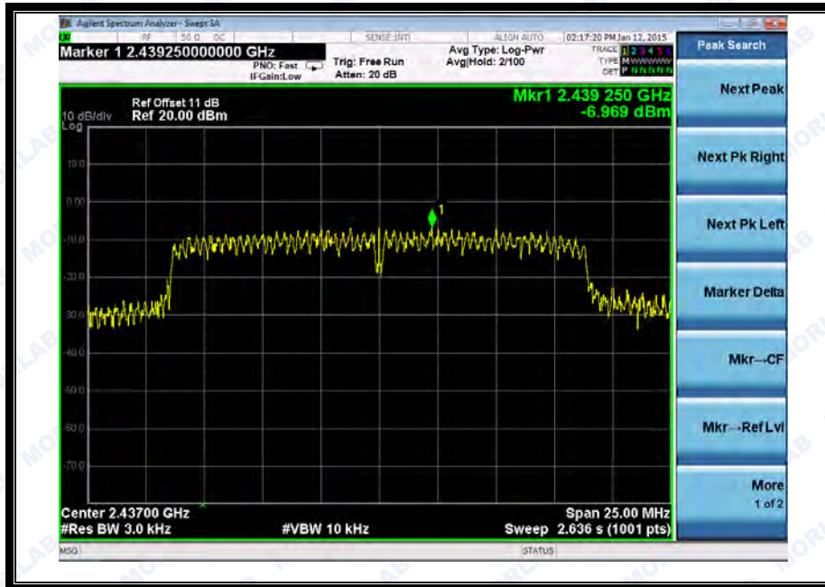
(Channel = 6 @ 802.11n-20MHz)
