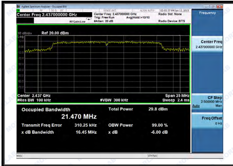
(Channel 6: 2437MHz @ 802.11g)
