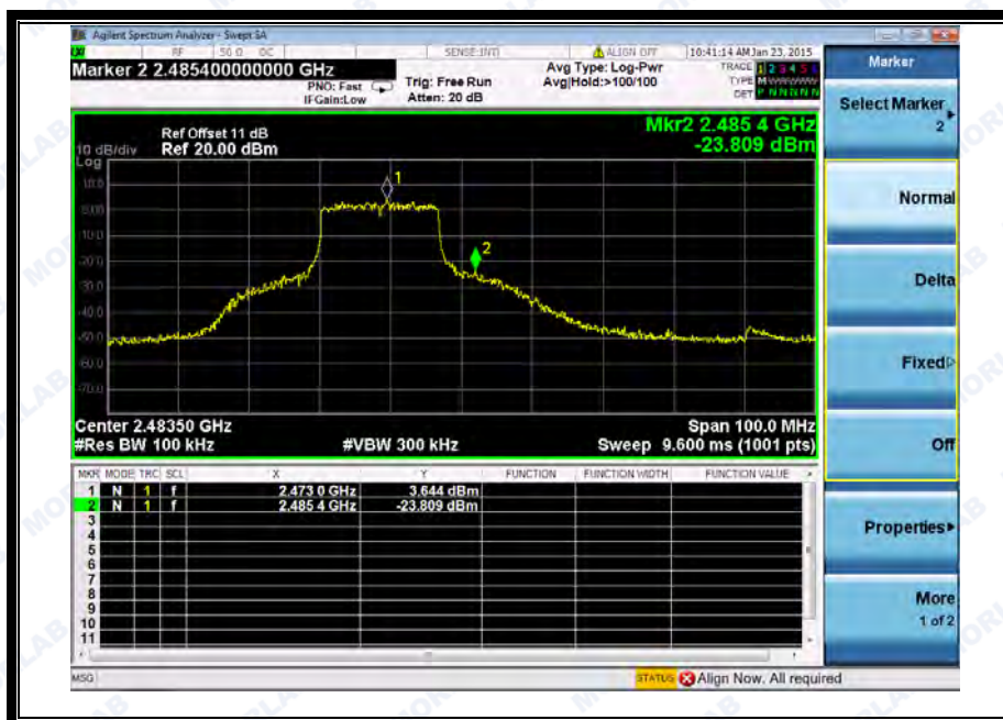
(Band Edge @ Channel = 11)
