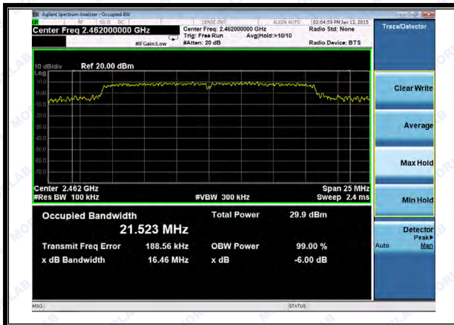
(Channel 11: 2462MHz @ 802.11g)
