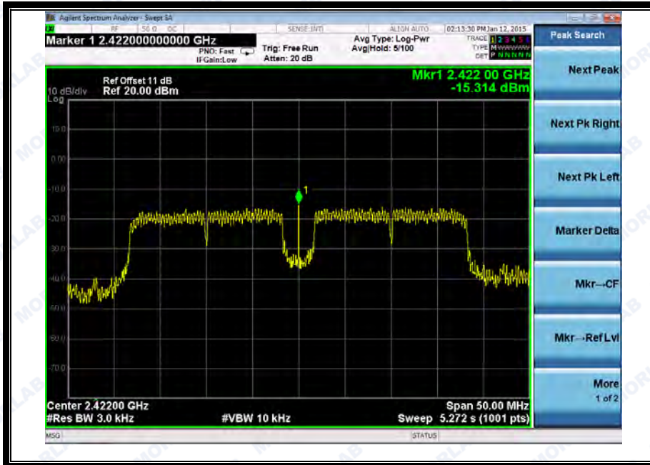
(Channel = 3 @ 802.11n-40MHz)
