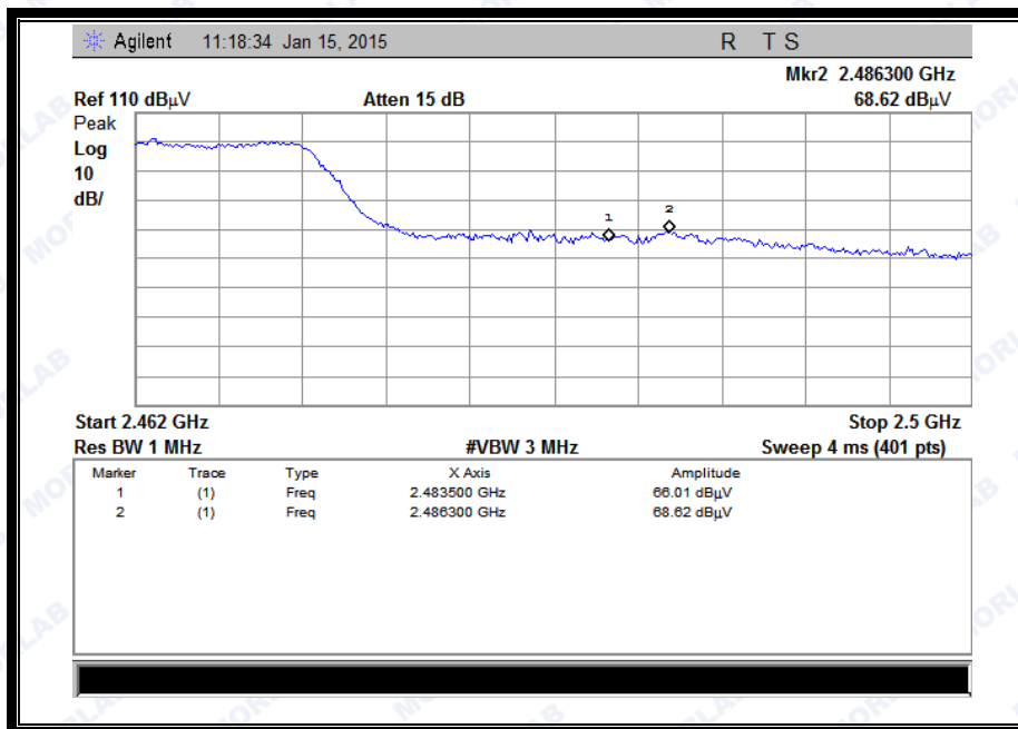
(Plot F1: Channel = 9 PEAK @ 802.11n-40)
