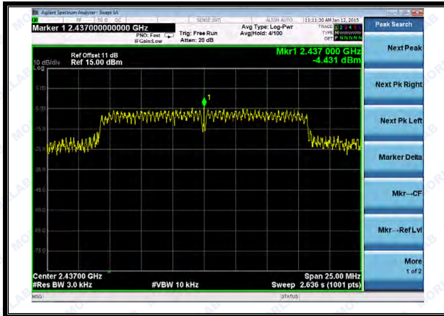
(Channel = 6 @ 802.11g)
