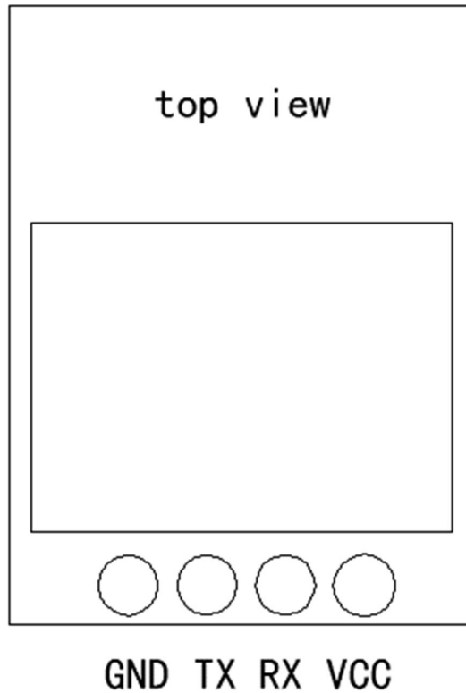
Figure 2.1. Terminal interface
