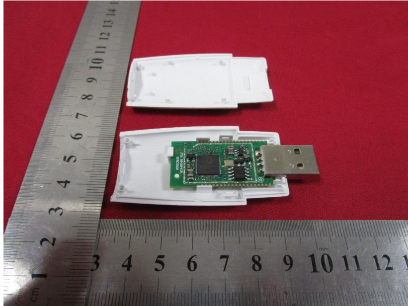
Internal photos of CE-SK103, US-SK103
