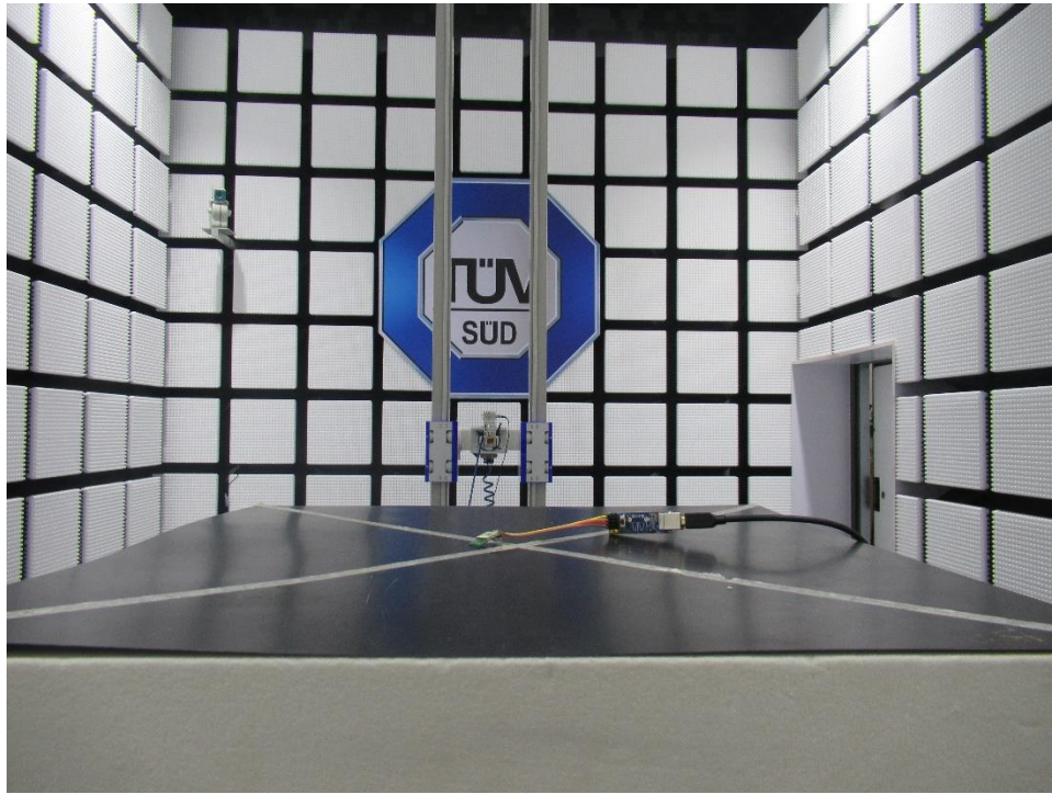
Radiated spurious emission 18GHz-40GHz
