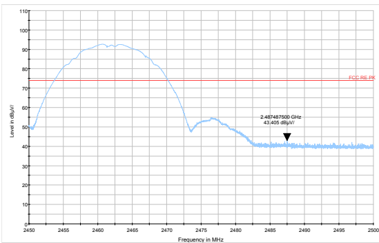
802.11b-Channel 11 Peak
